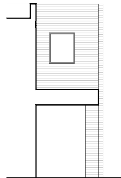
PRE-EXISTING SIDE ELEVATION 1:100
