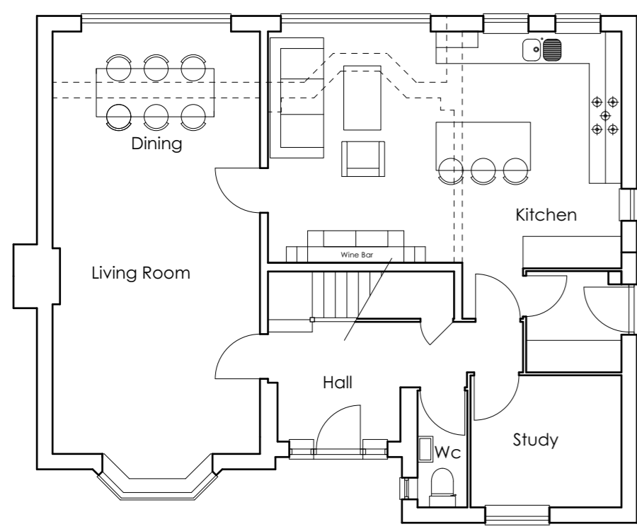
Ground Floor Plan Option1
