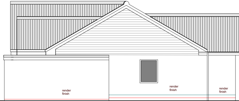
side garage elevation
