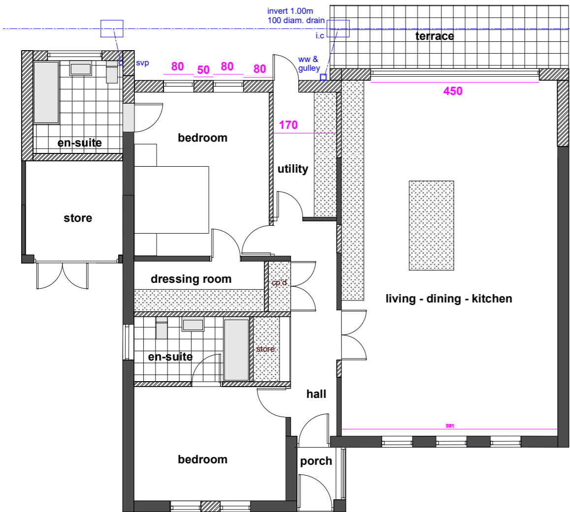
floor layout
