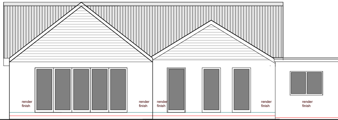
rear elevation
