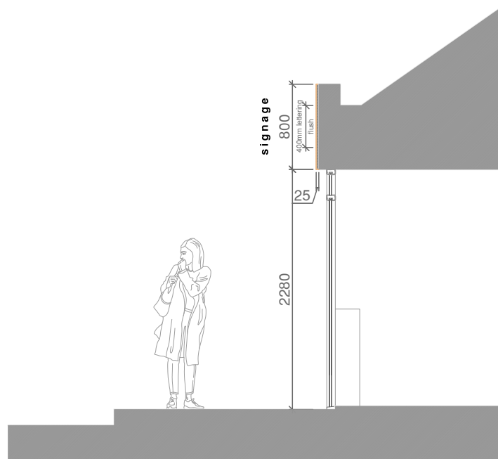
SECTION THROUGH EXISTING SIGN SCALE 1/50
