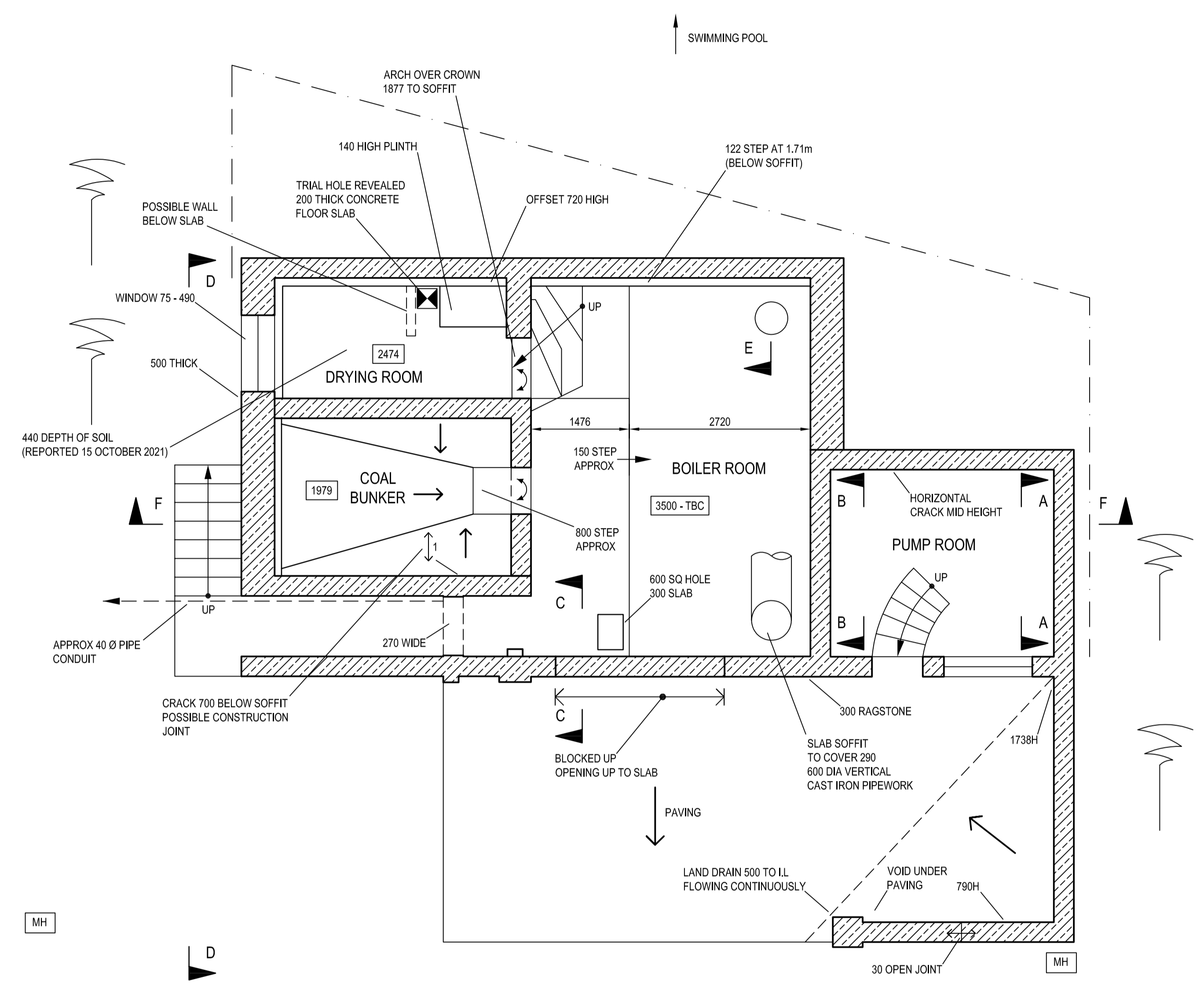
PUMPING STATION PLAN SCALE 1:50
