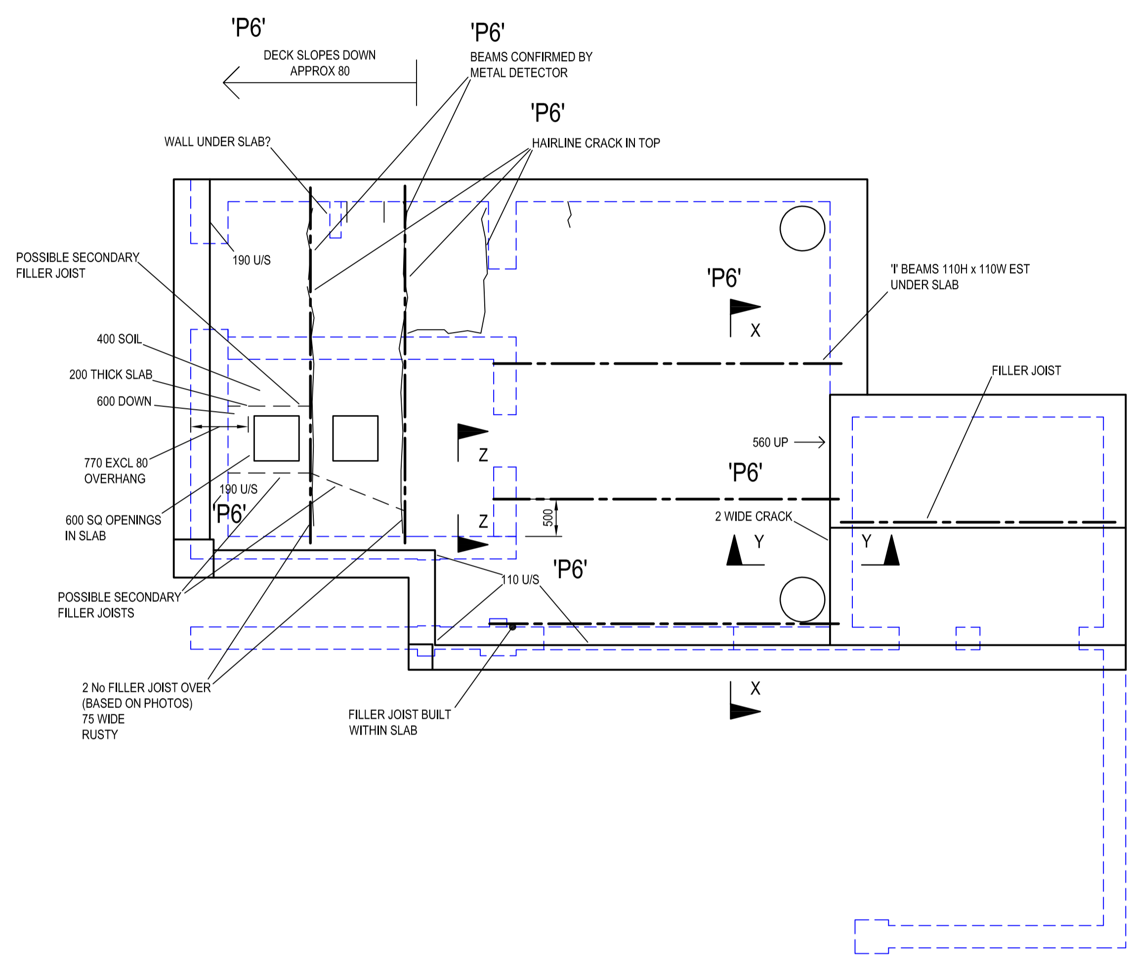
PUMPING STATION ROOF PLAN SCALE 1:50
