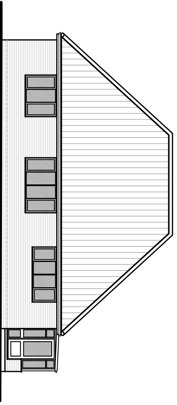
EXISTING REAR ELEVATION (1:100)
