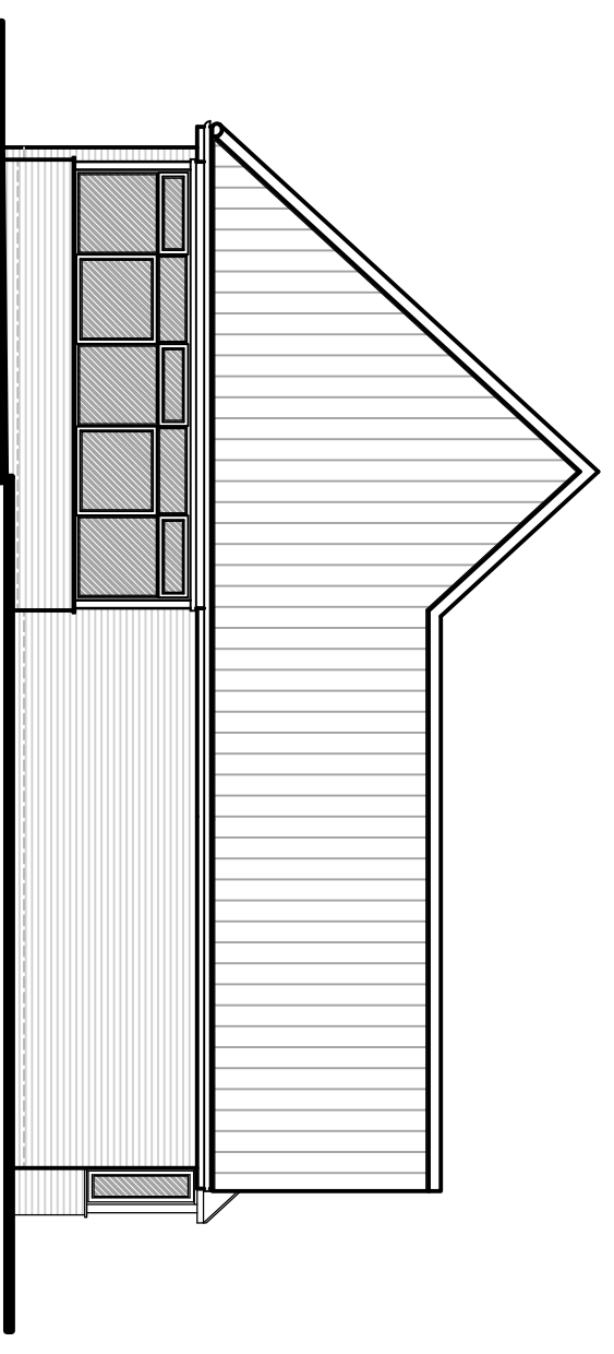
EXISTING SIDE ELEVATION (1:100)
