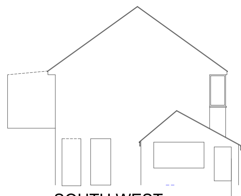
SOUTH WEST 1:100 0 1m 2m 3m 4m
