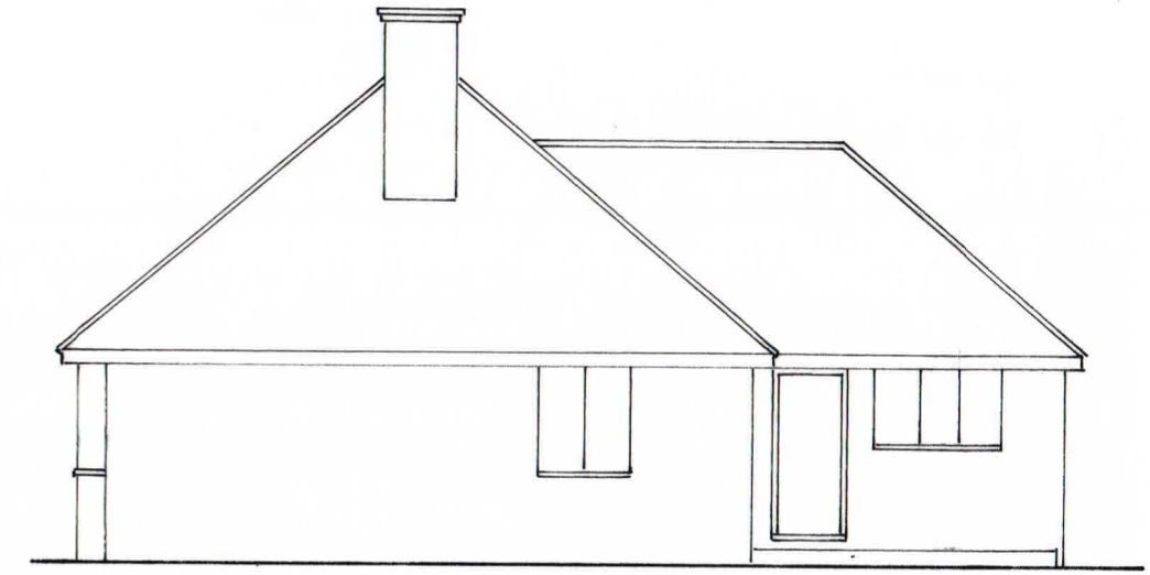
South Elevation
