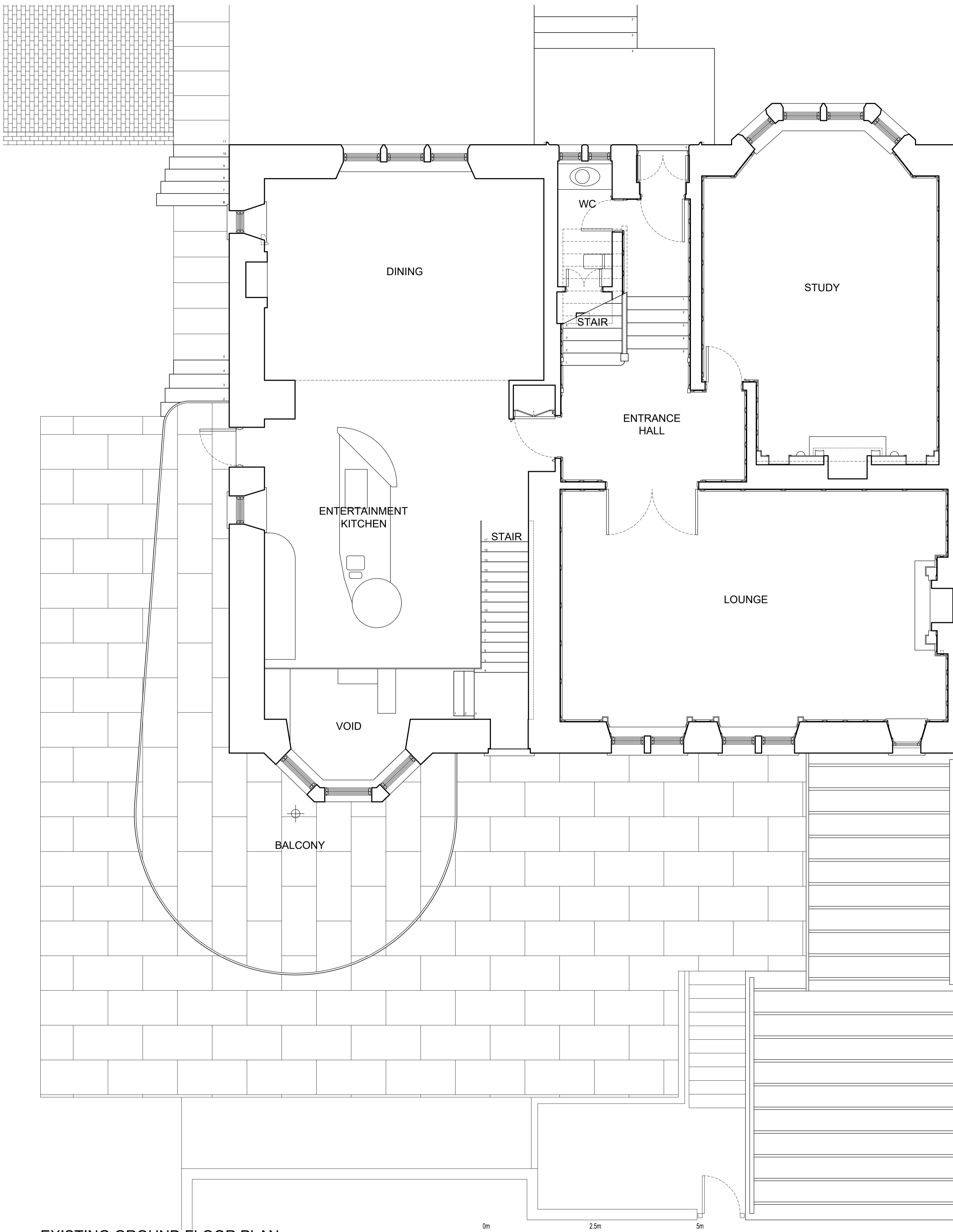
EXISTING GROUND FLOOR PLAN
