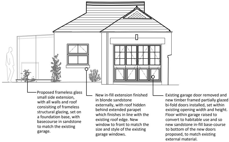
PROPOSED FRONT GARAGE ELEVATION // 1:100
