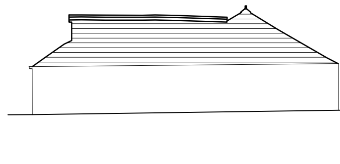
PROPOSED BOUNDARY SIDE GARAGE ELEVATION // 1:100
