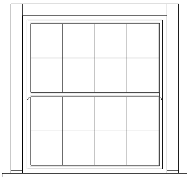
WINDOW 2 Ground floor front elevation
