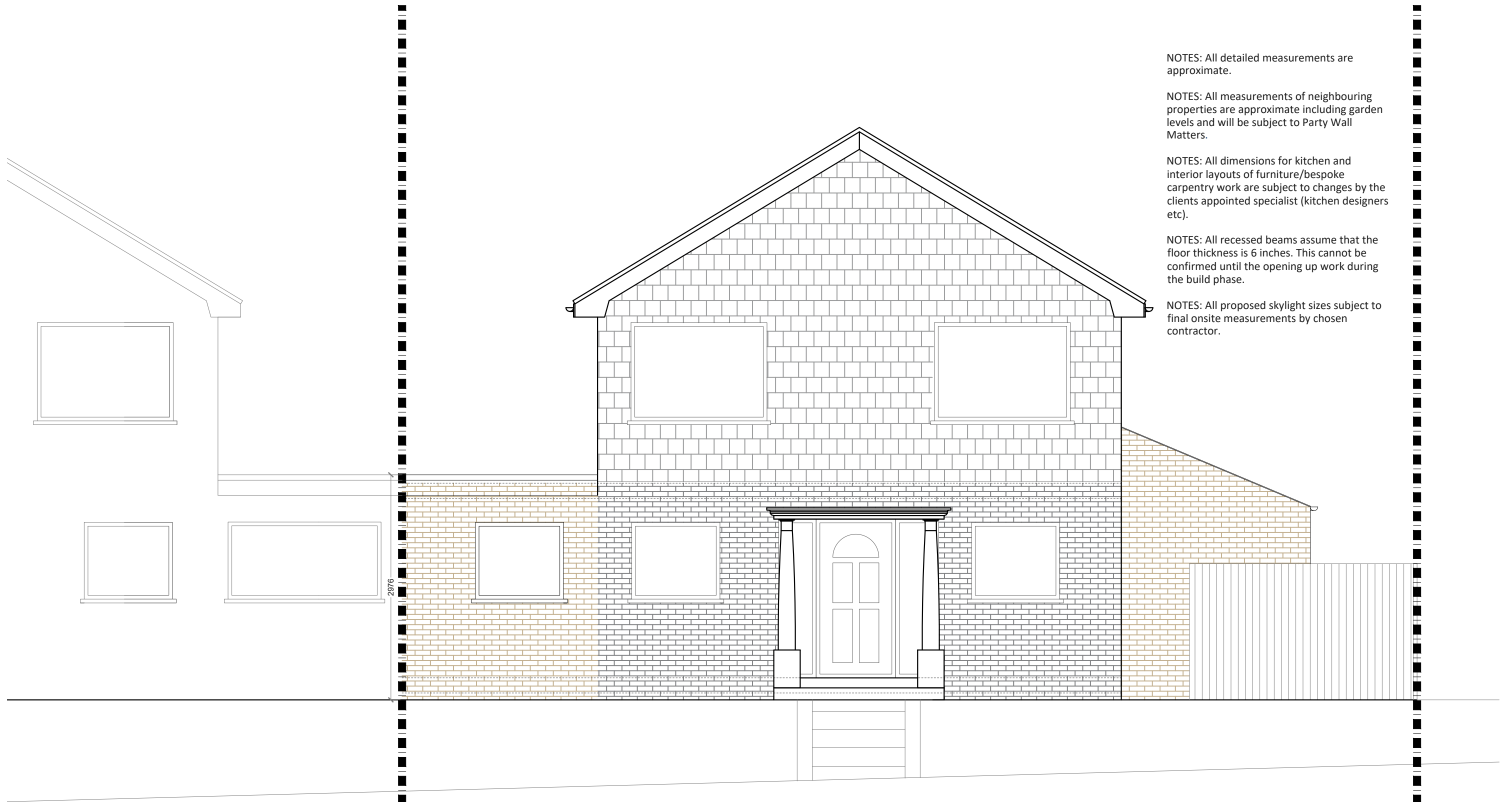
PROPOSED FRONT ELEVATION SCALE 1:50
