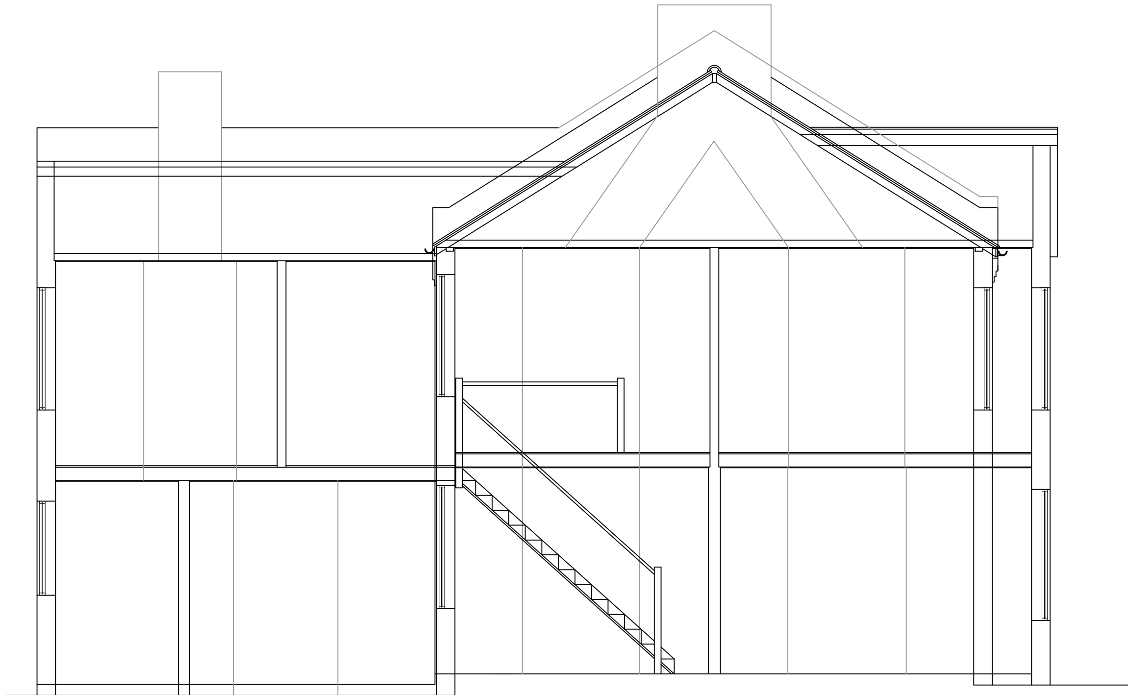
EXISTING SECTION (SIDE)
