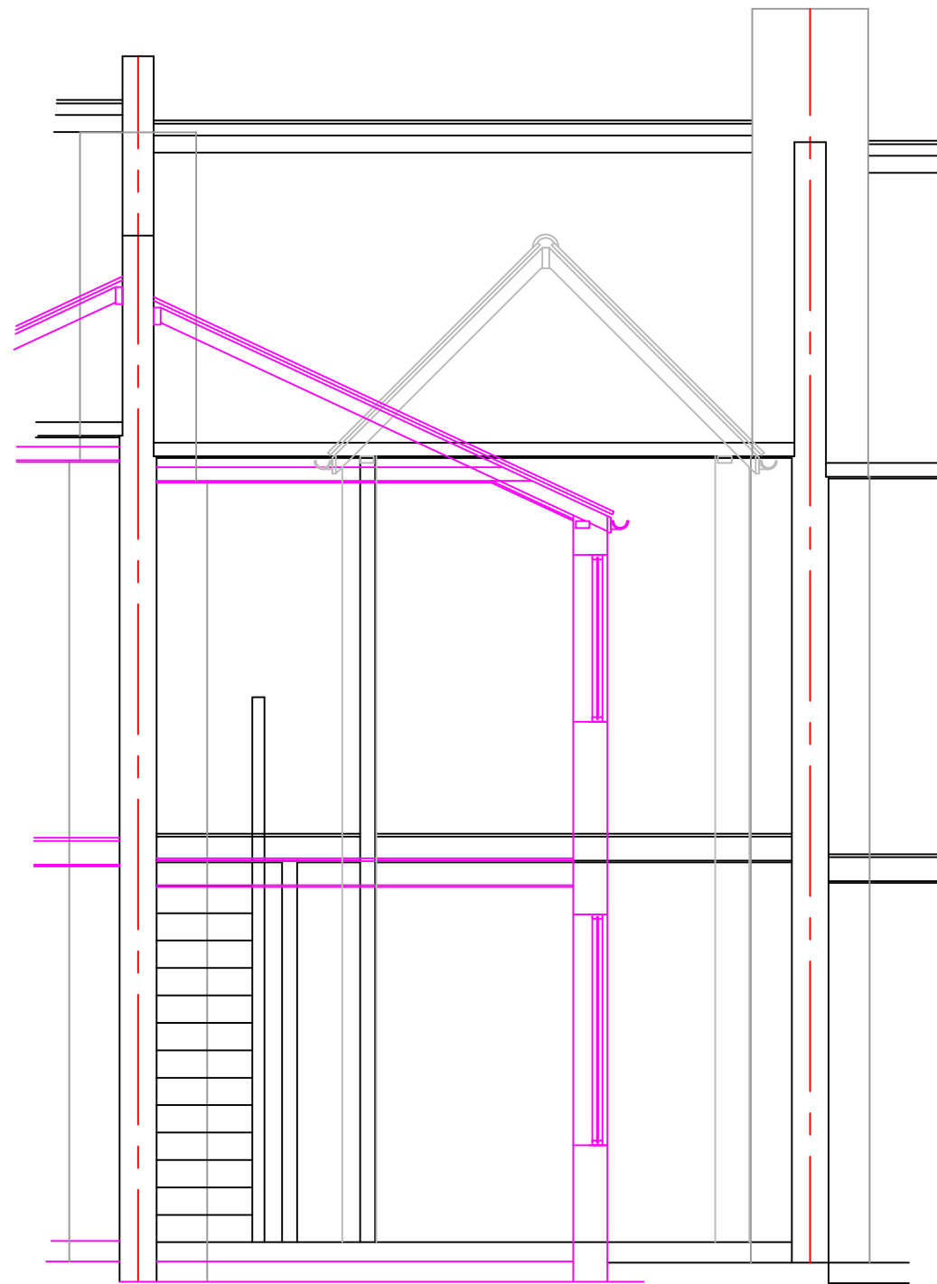
EXISTING SECTION (REAR TO FRONT)
