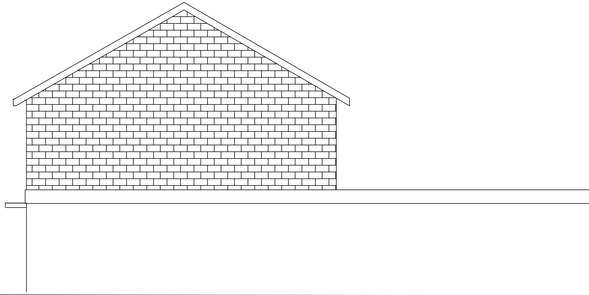
SIDE ELEVATION NE (PROPOSED)
