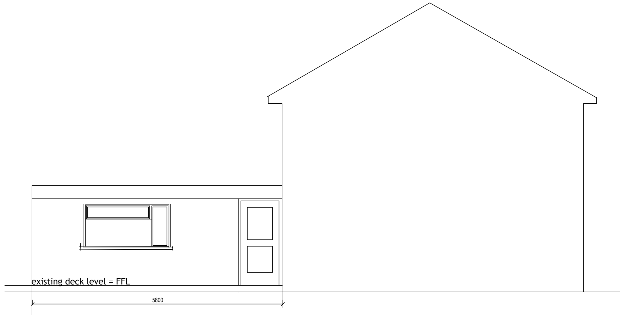
SIDE ELEVATION SW (PROPOSED)
