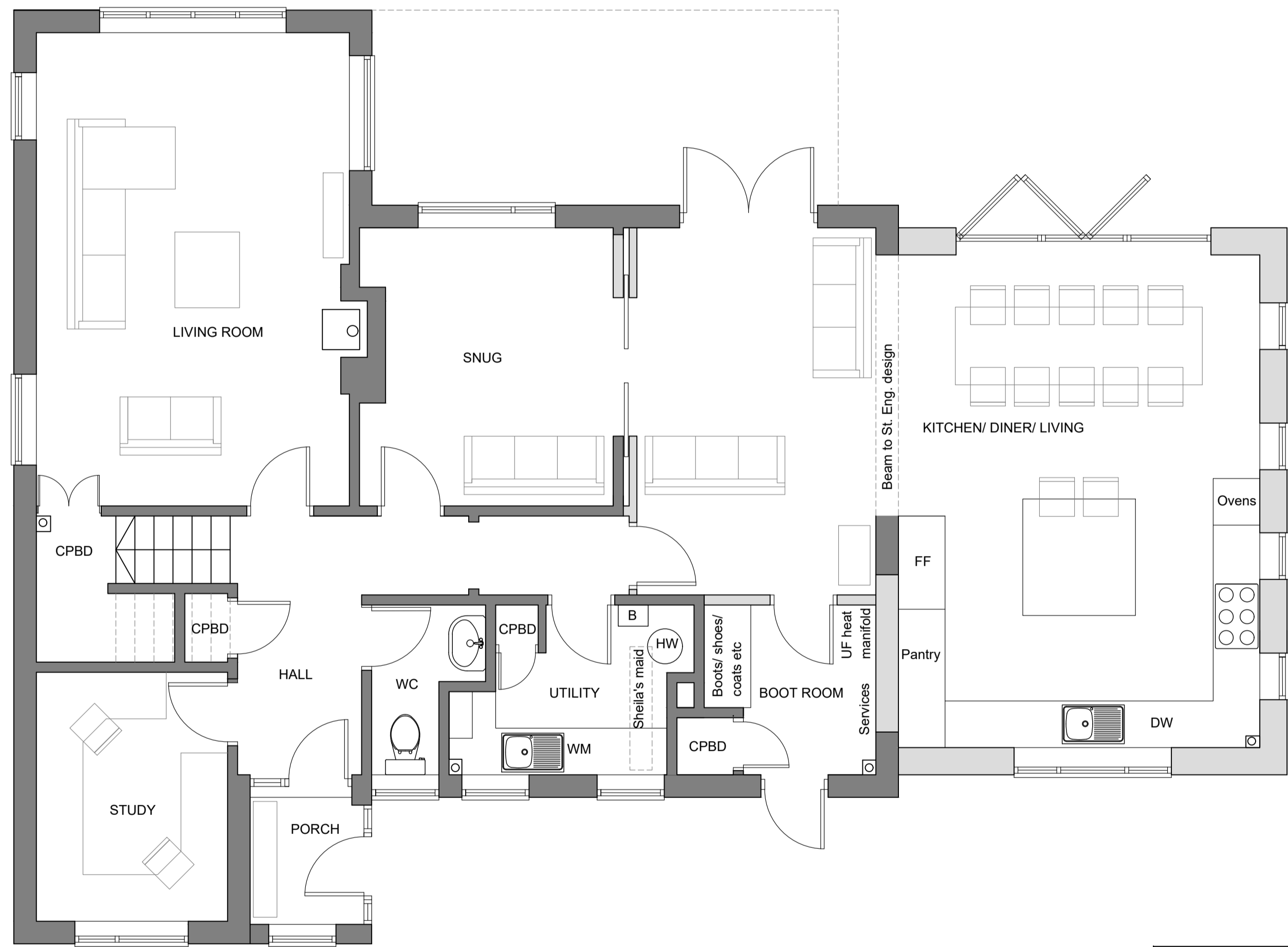
GROUND FLOOR
