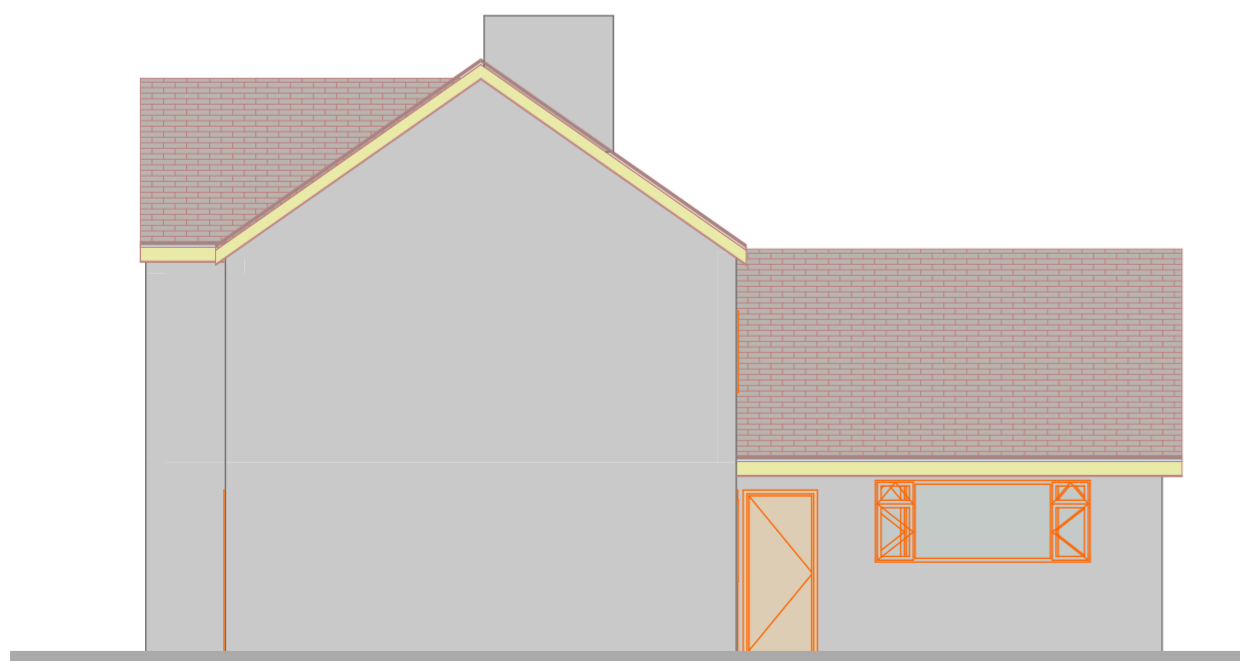
6 Side elevation 1:100
