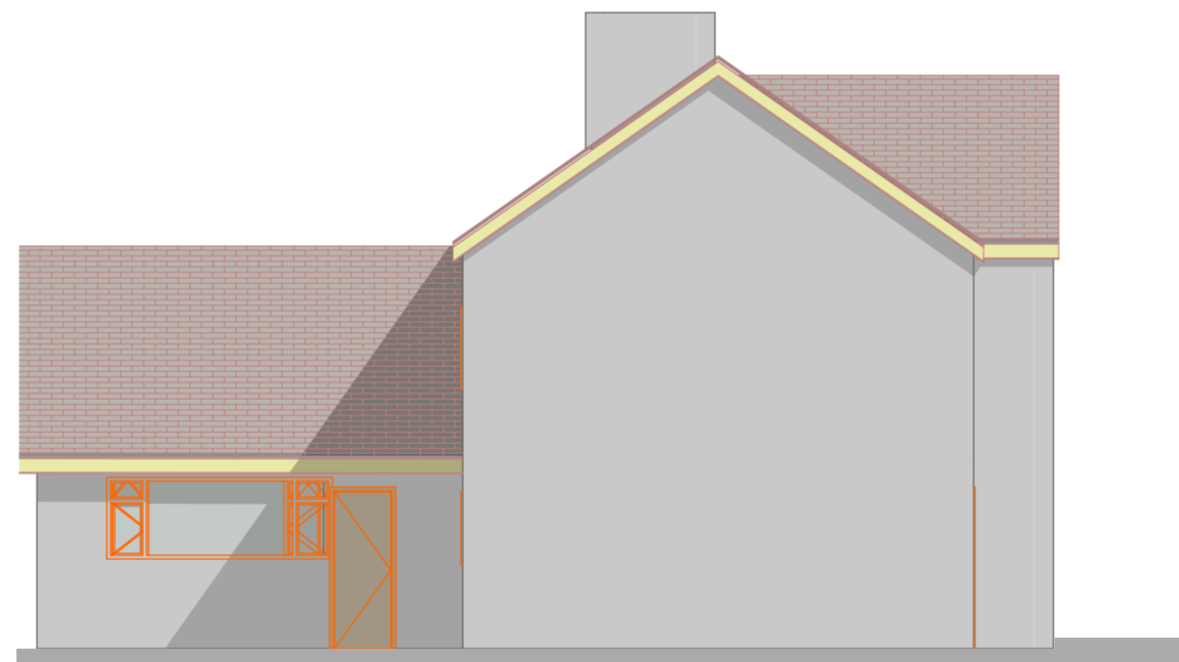
5 Side elevation 1:100
