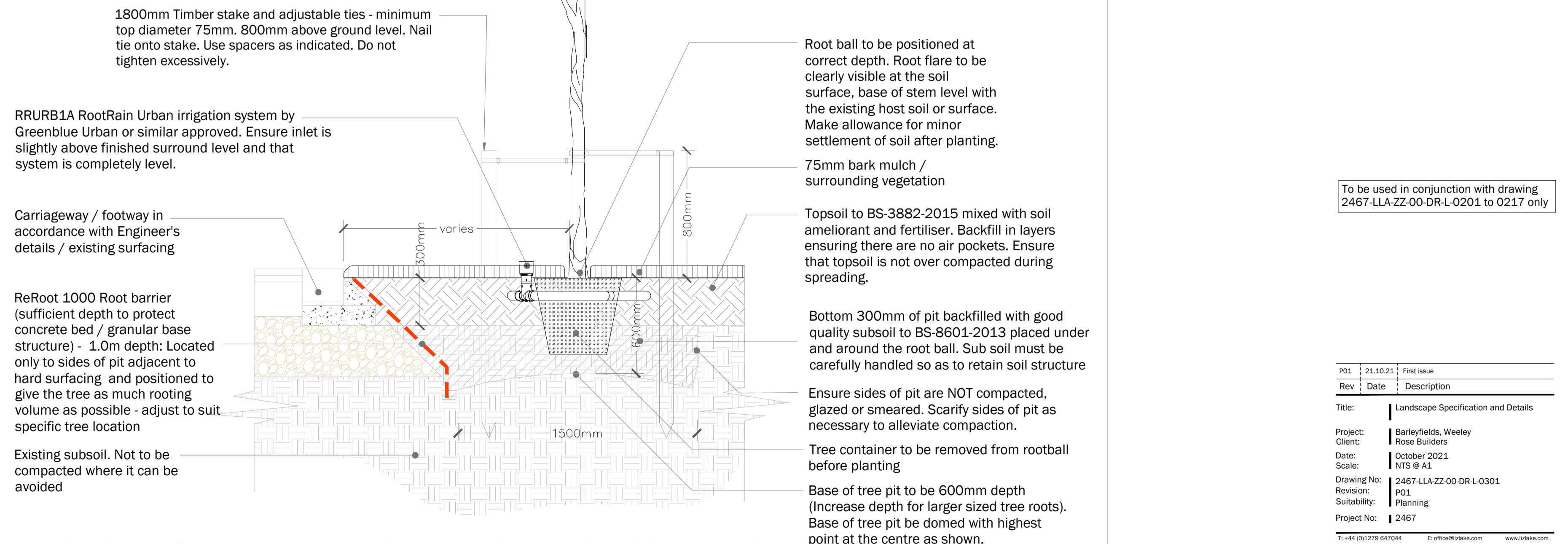
TYPICAL CLEAR STEM TREE PLANTING DETAIL FOR TREES IN CONTAINERS Double stake fixing in soft landscape adjacent to Carriageway / footway - Not to Scale
