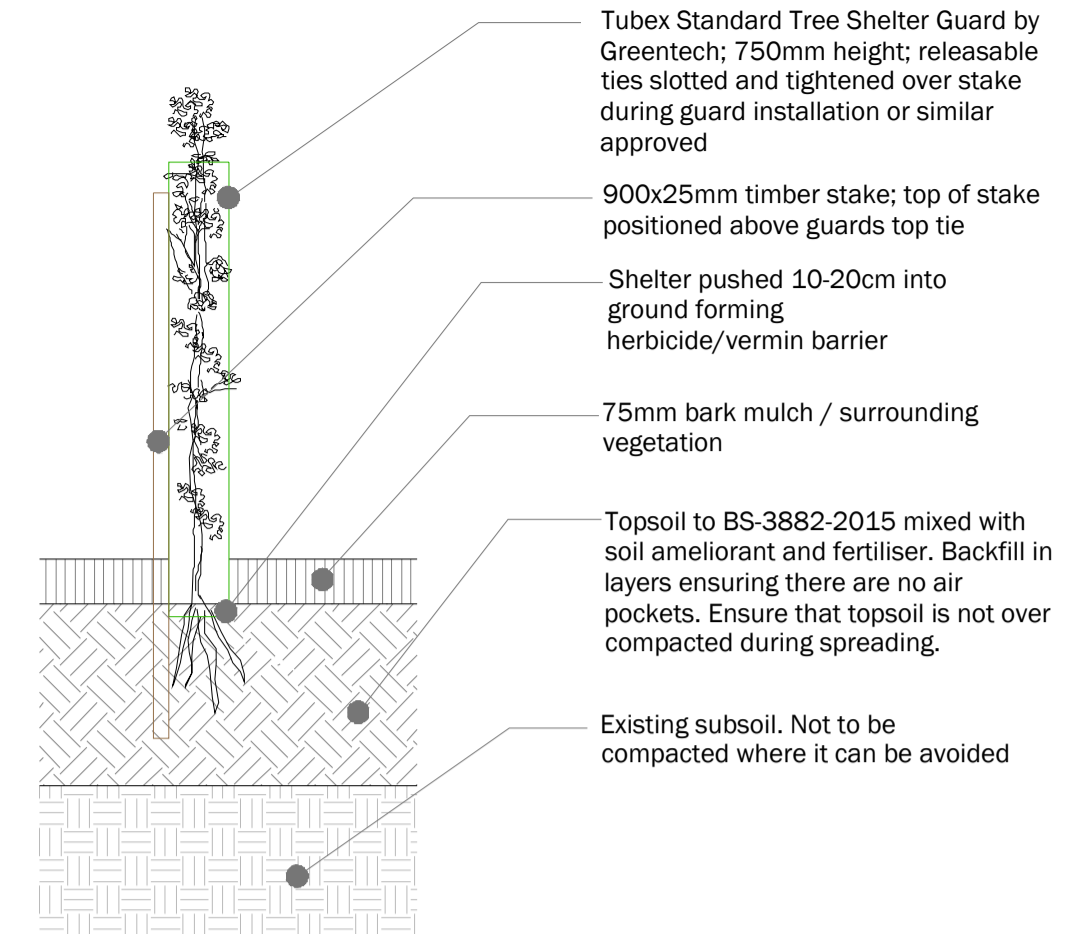
NATIVE HEDGE PLANTING DETAIL
