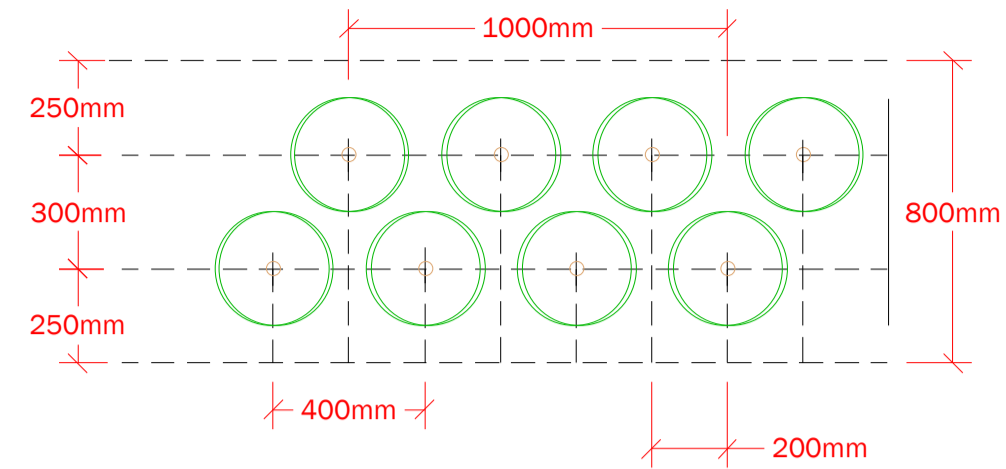
DOUBLE STAGGERED HEDGE PLANTING DETAIL; 5 per metre; For mixed native hedging
