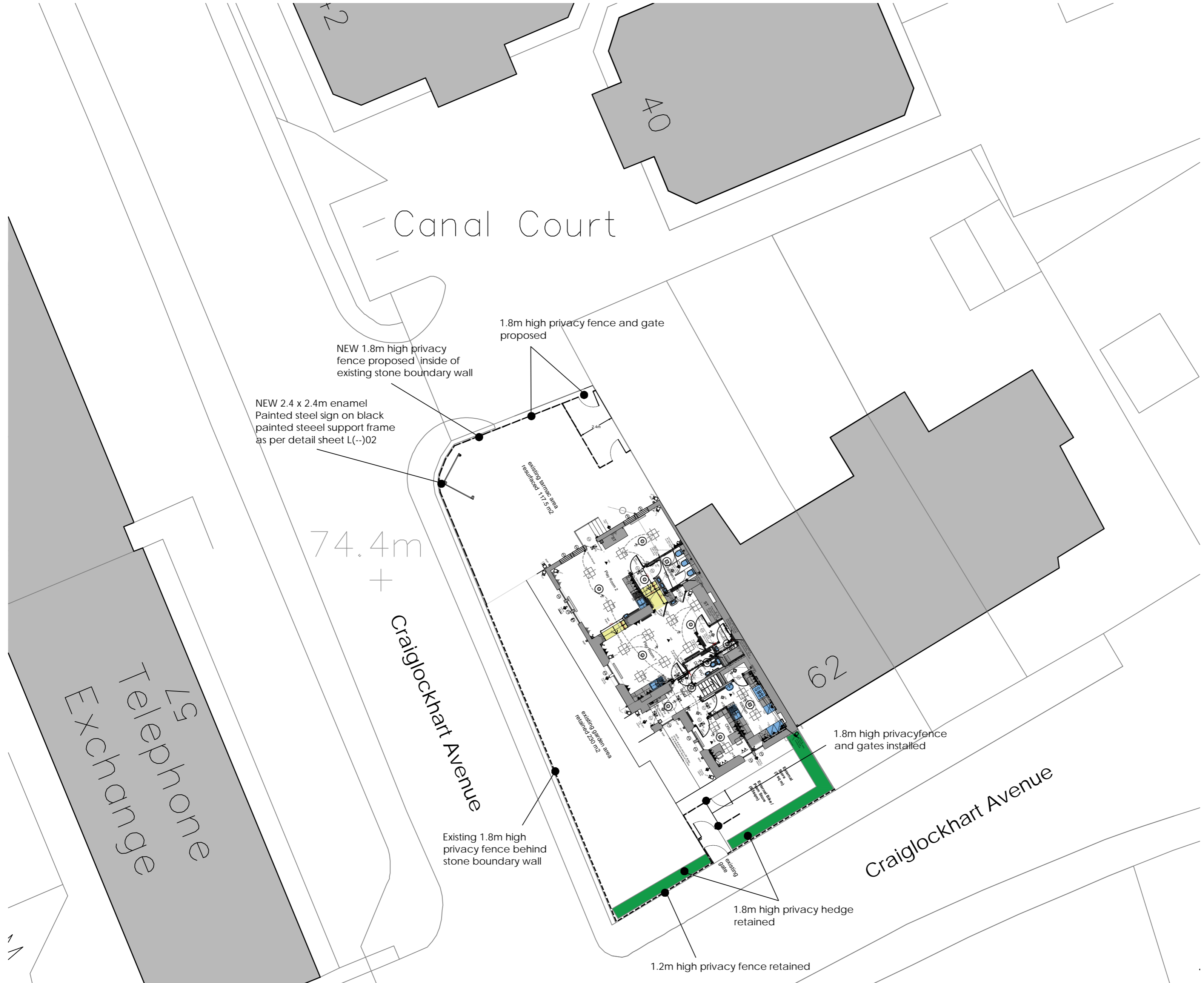
SITE PLAN - AS PROPOSED 1:200 @A2
