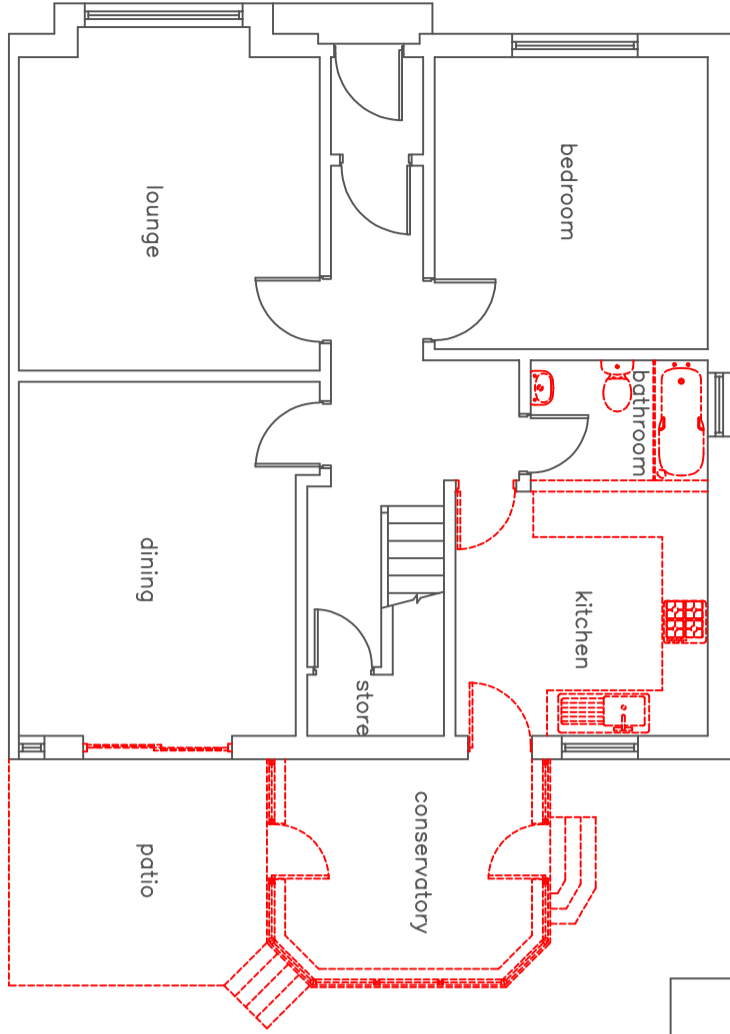
Existing Ground Floor Plan Scale:- 1:100 (removdis shown red dashed)
