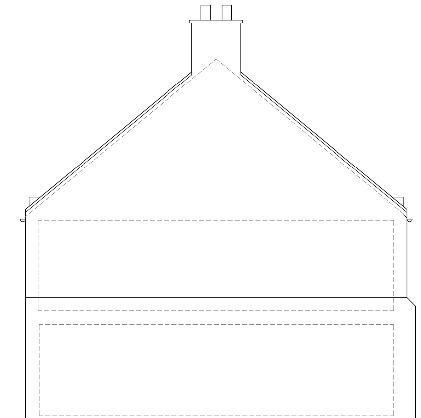
Existing Gable Elevation 1:100
