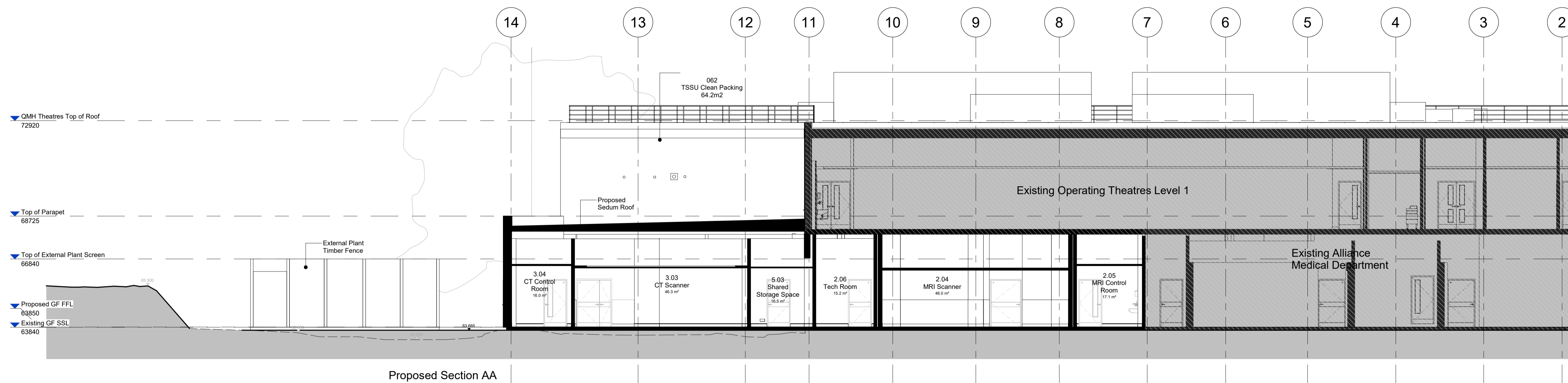
Proposed Section AA
