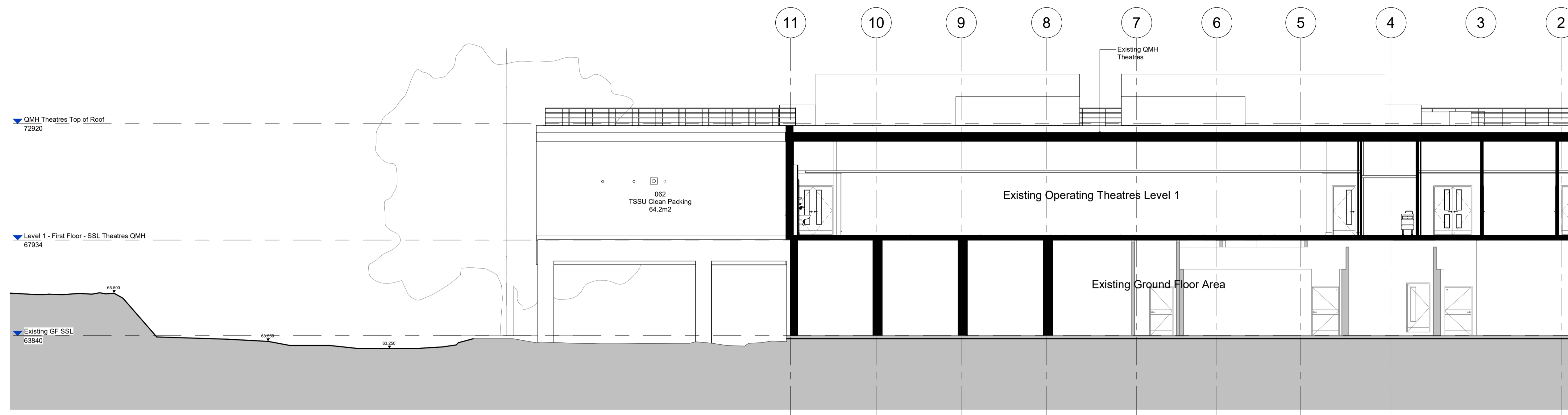
Existing Site Section AA
