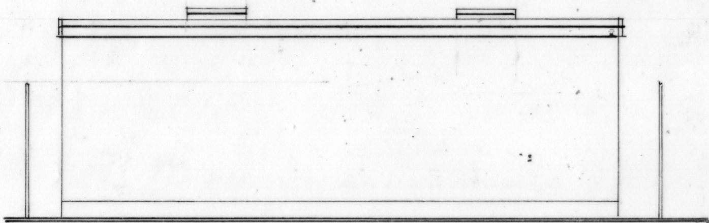
Rear Elevation
