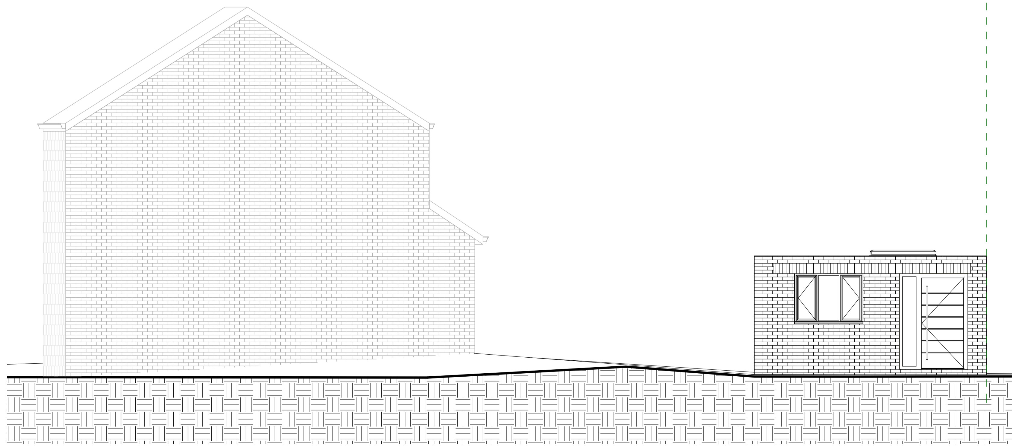
3 Front Proposed 1 : 50
