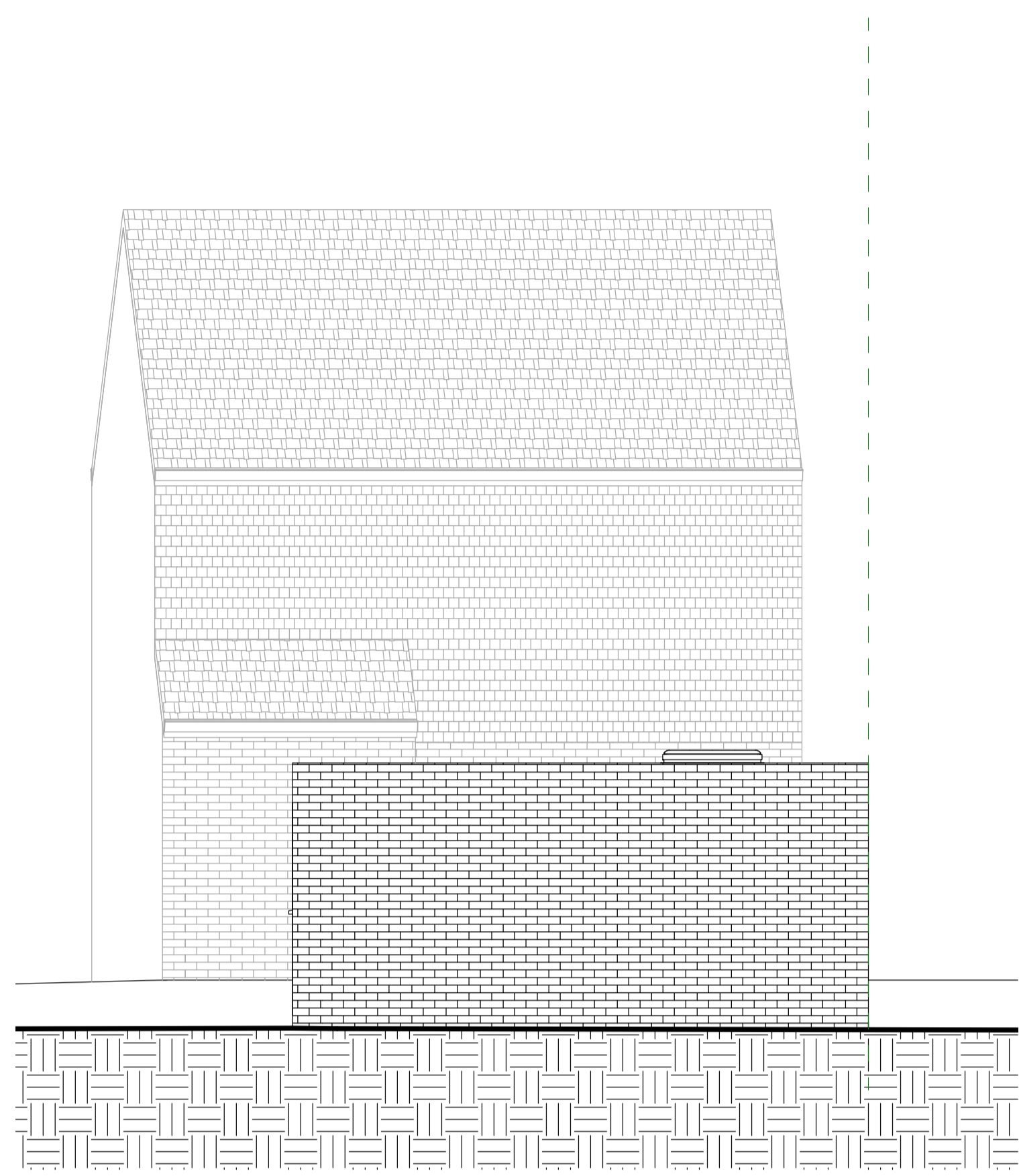
2 Flank 2 Proposed 1 : 50
