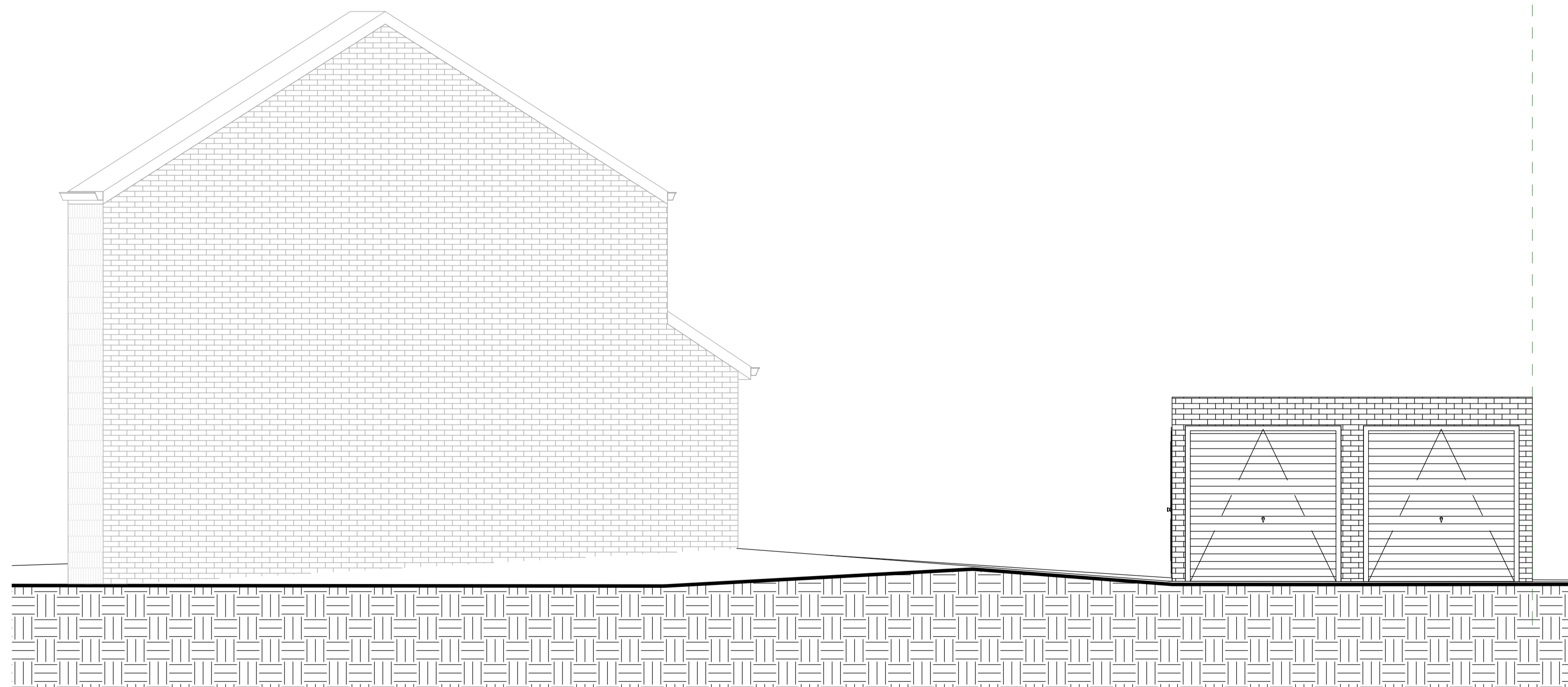
3 Front Existing 1 : 50
