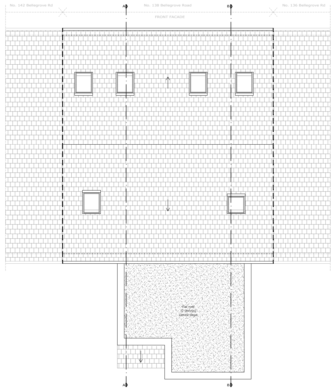
PROPOSED ROOF
