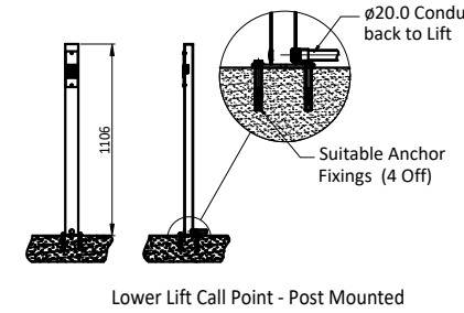
Lower Lift Call Point - Post Mounted
