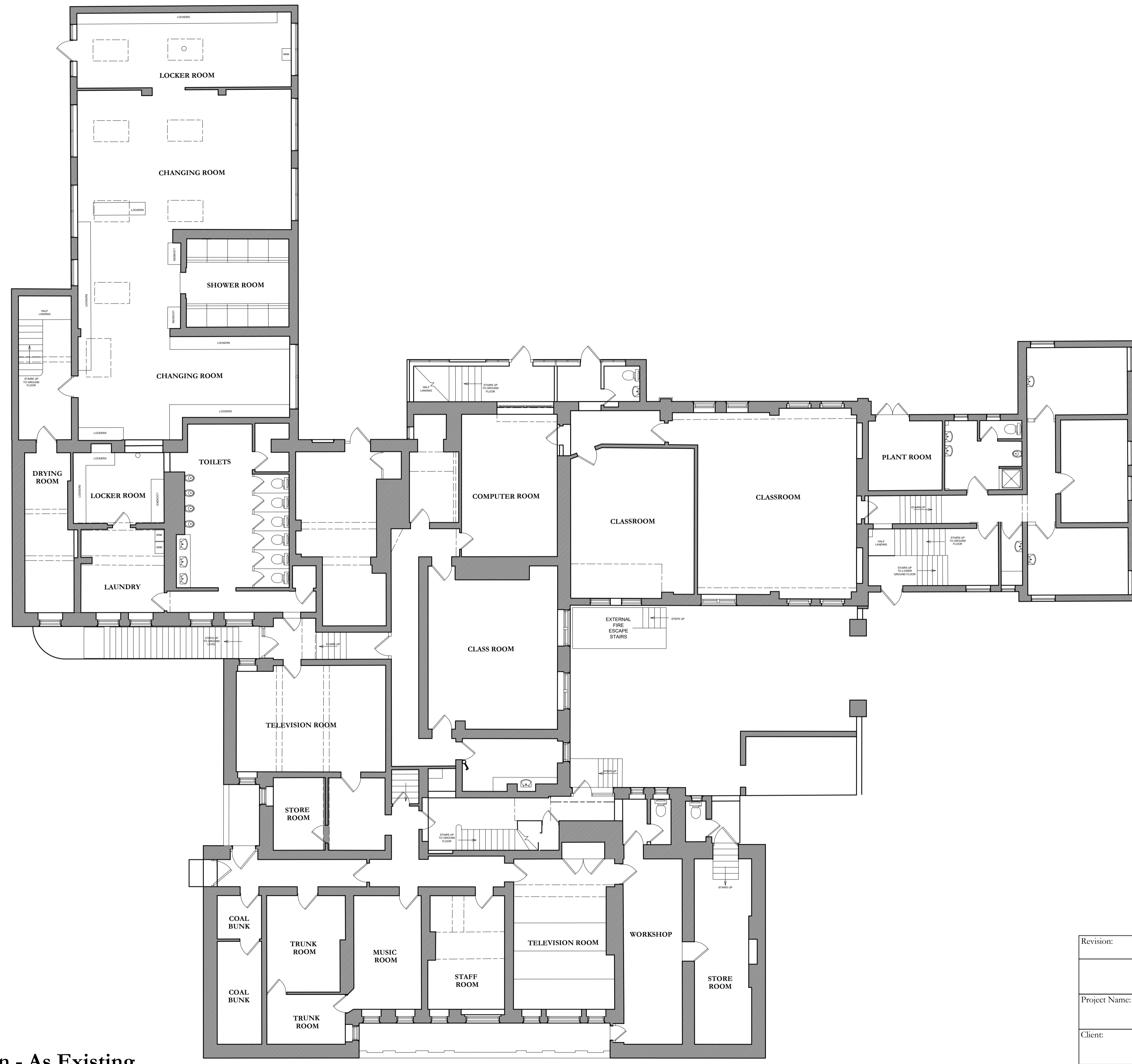
Lower Ground Floor Plan - As Existing 1:200 @ A3
