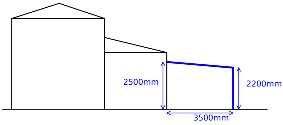
West elevation, 1:100 New veranda shown in blue Roof in clear polycarbonate, rafters and supports white aluminium
