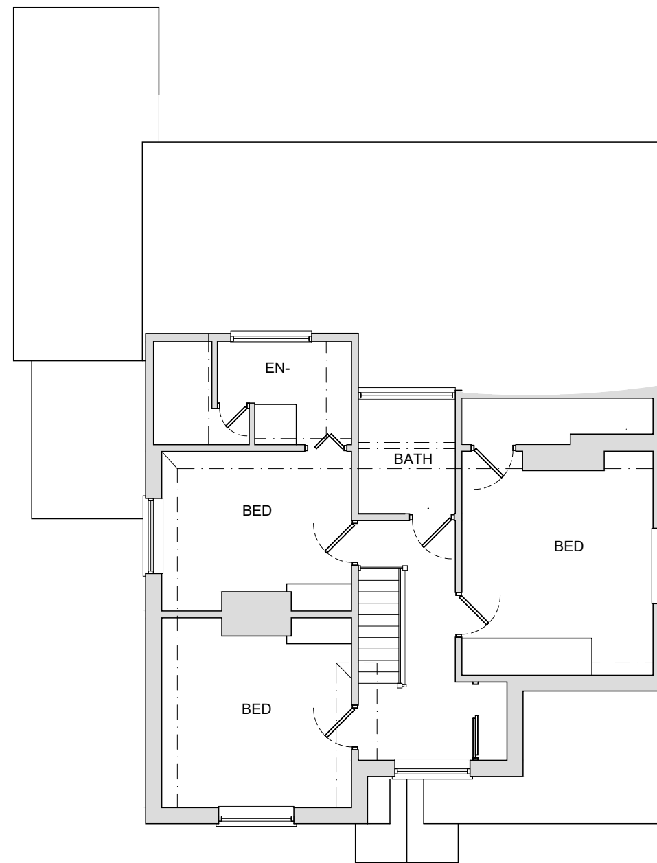
FIRST FLOOR 1:100
