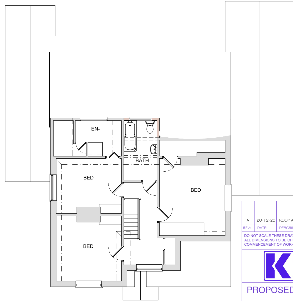
FIRST FLOOR 1:100
