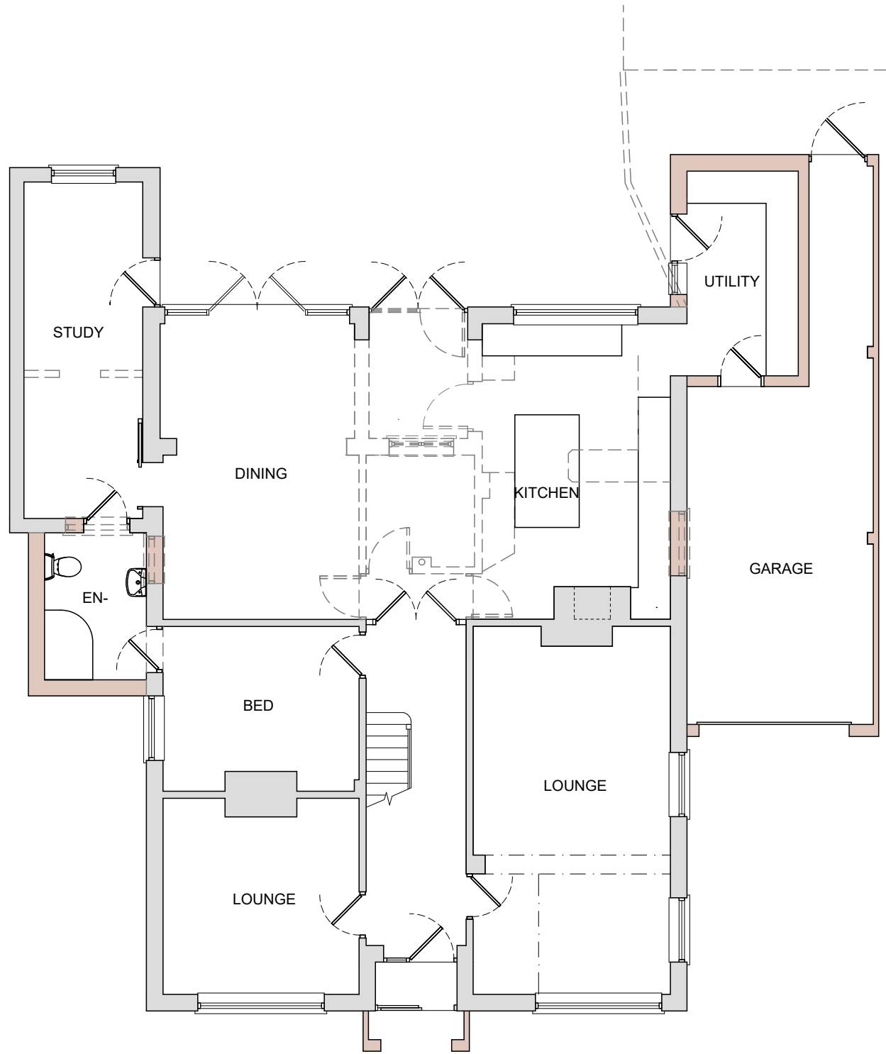
GROUND FLOOR 1:100
