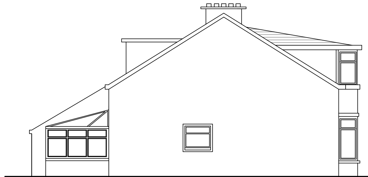
SIDE ELEVATION
