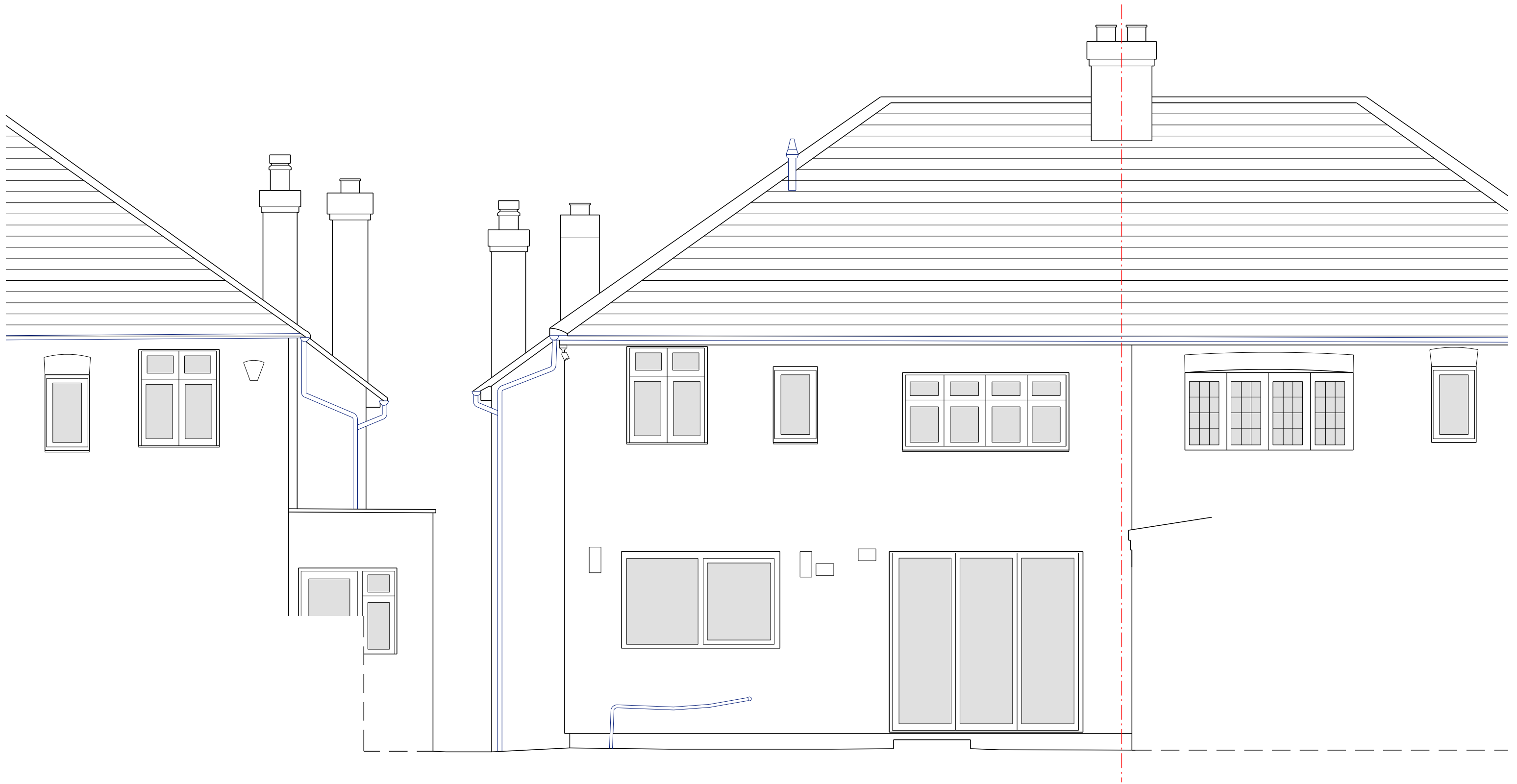
01 Existing Rear Elevation 1:50@A3
