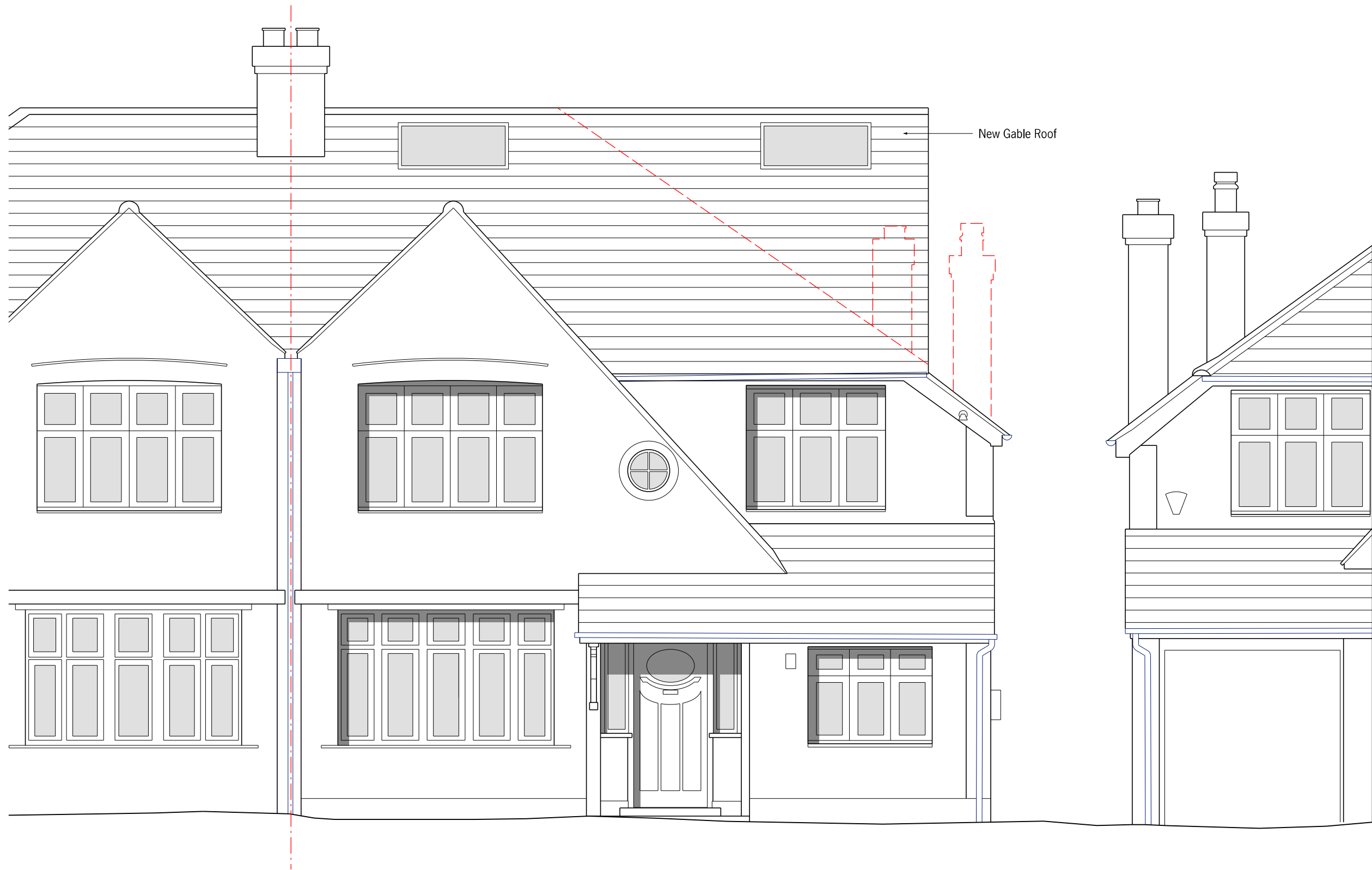
01 Proposed Front Elevation 1:50@A3
