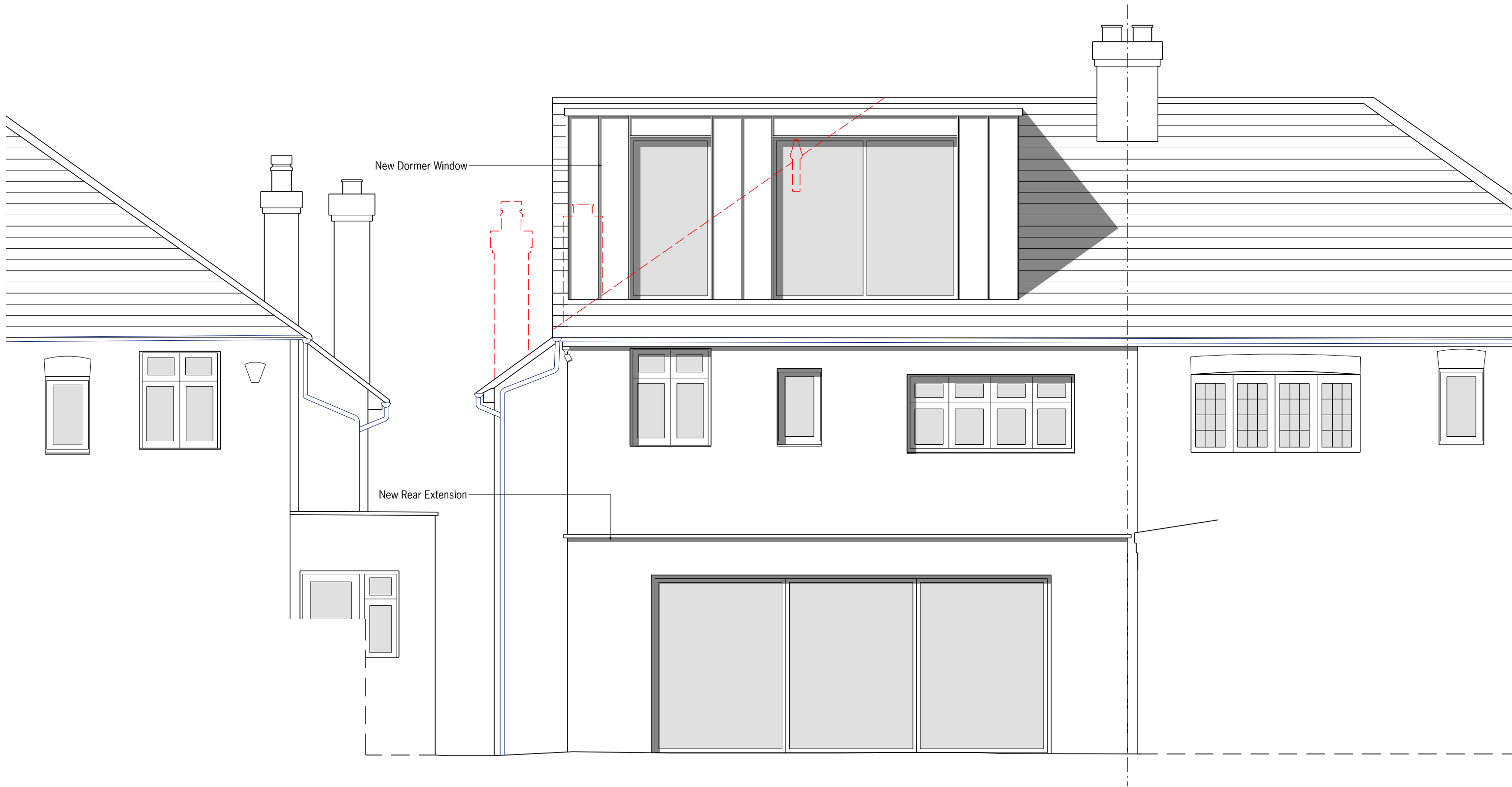
01 Proposed Rear Elevation 1:50@A3
