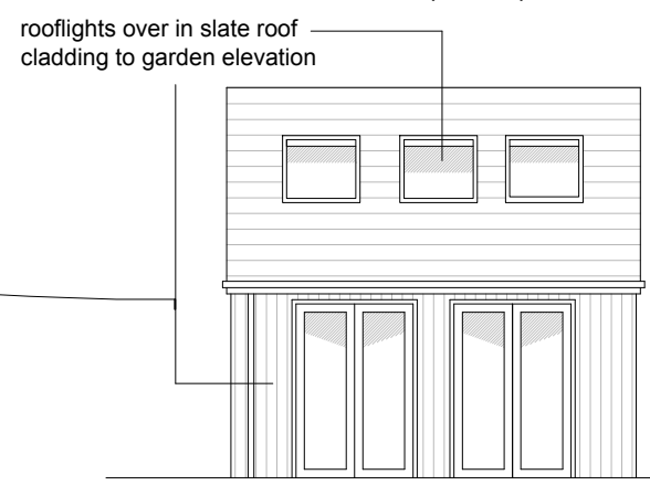
PROPOSED GARDEN ELEVATION (SOUTH)
