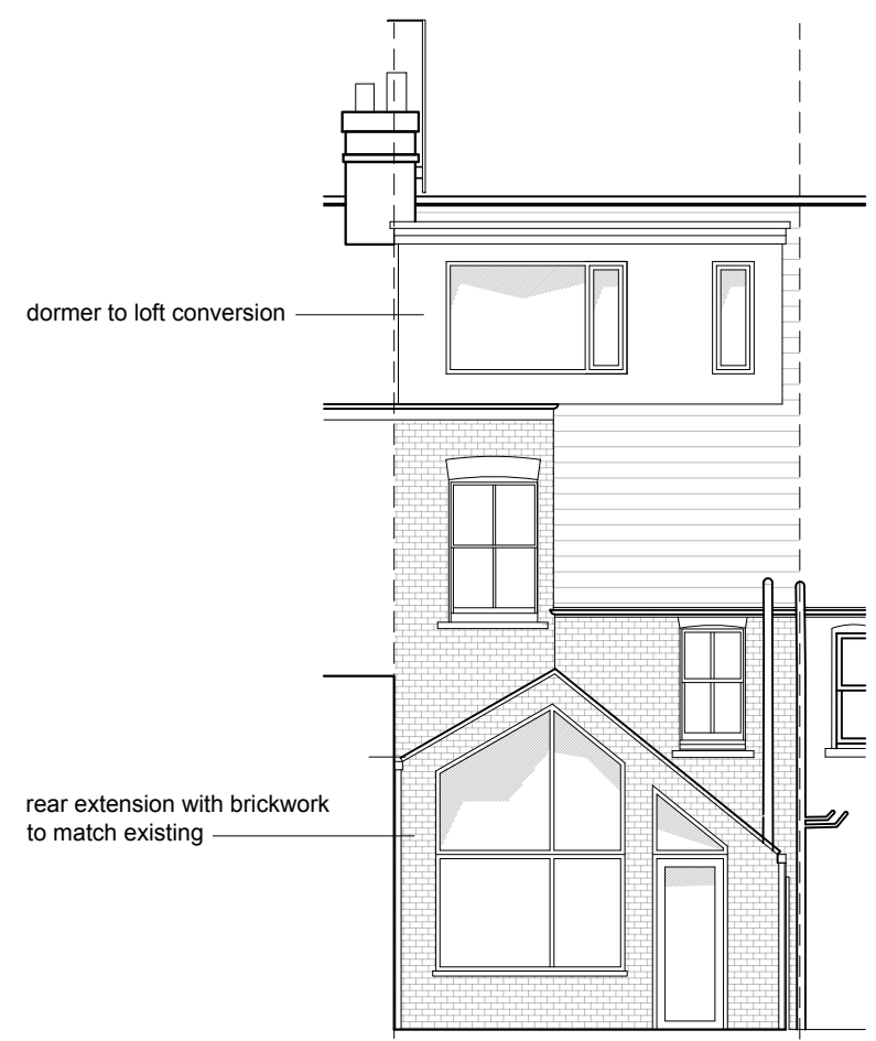
PROPOSED GARDEN ELEVATION
