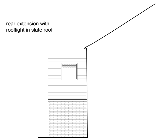
PROPOSED PART SIDE ELEVATION
