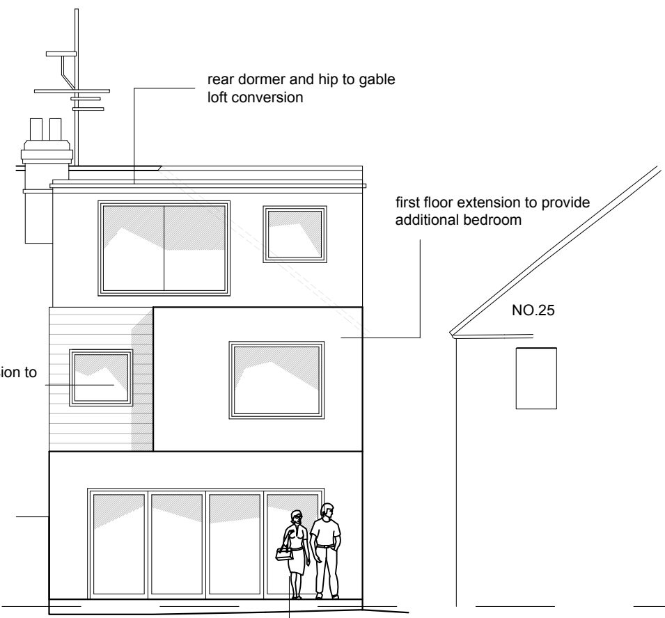
EAST (GARDEN) ELEVATION
