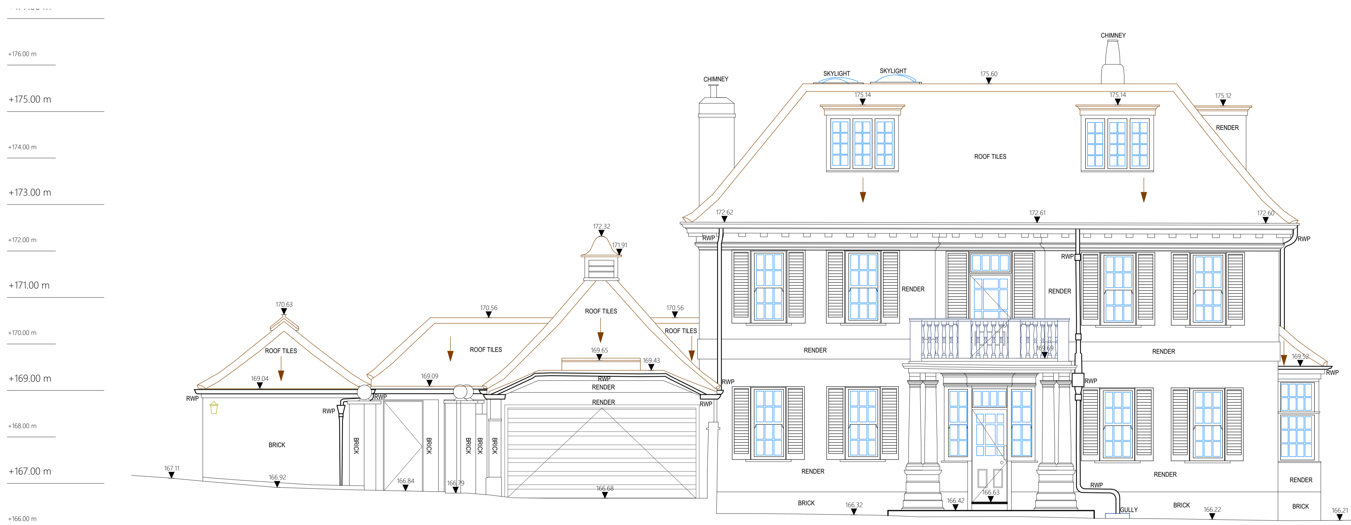
D MEASURED SURVEY - ELEVATIONS 1:50
