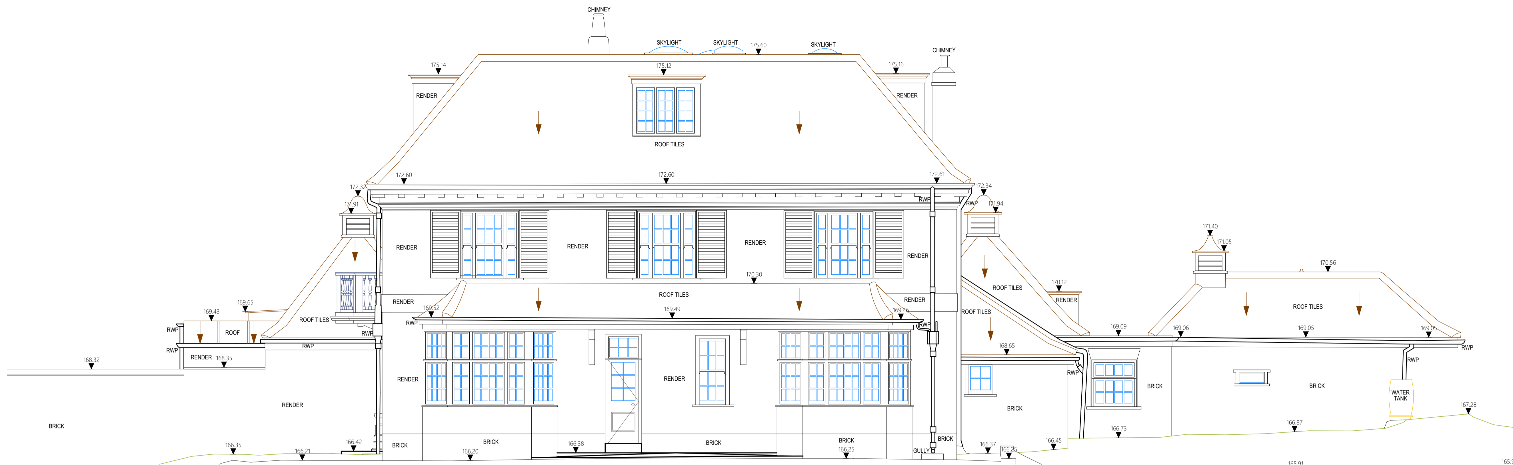
MEASURED SURVEY - ELEVATIONS
