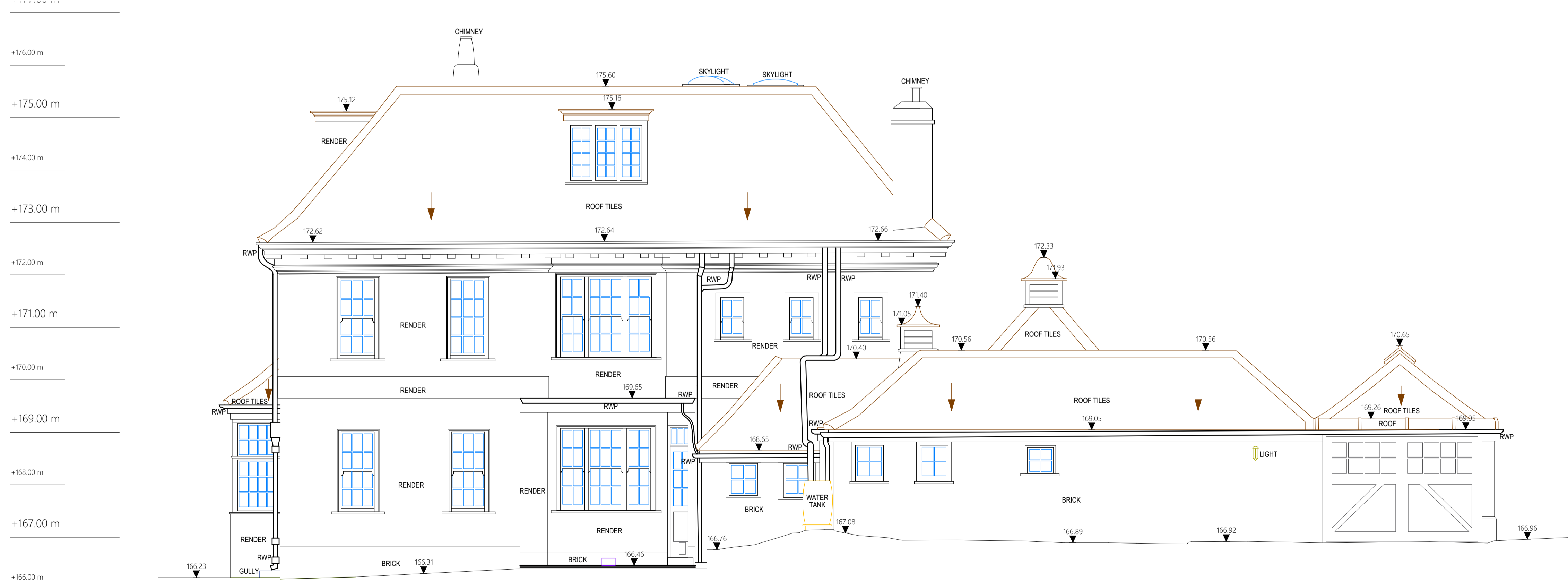
MEASURED SURVEY - ELEVATIONS
