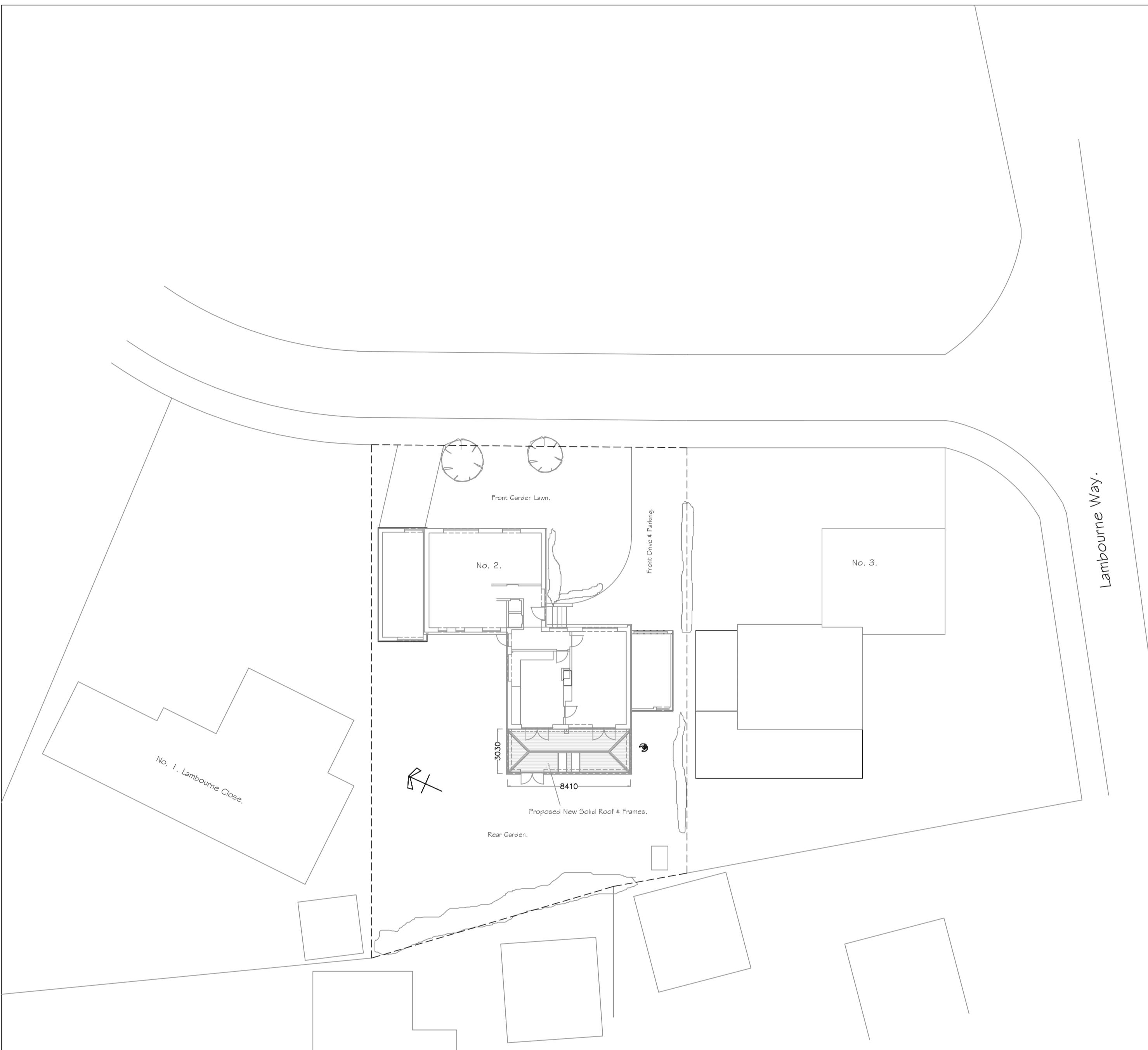
PROPOSED SITE BLOCK PLAN 1/200. Read in conjunction with 1/1250 Location plan.
