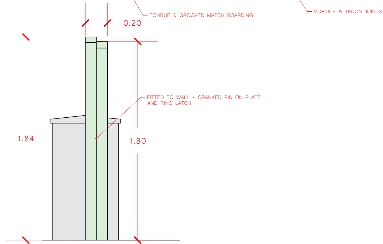
PROPOSED SOUTH-NORTH GATE SECTION
