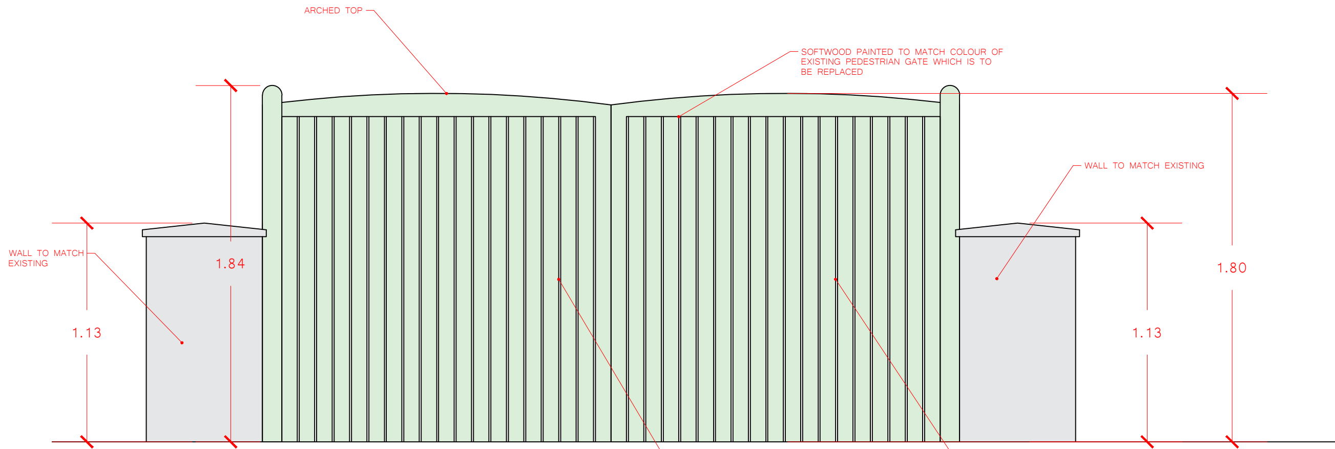
PROPOSED WEST-EAST GATE DETAIL
