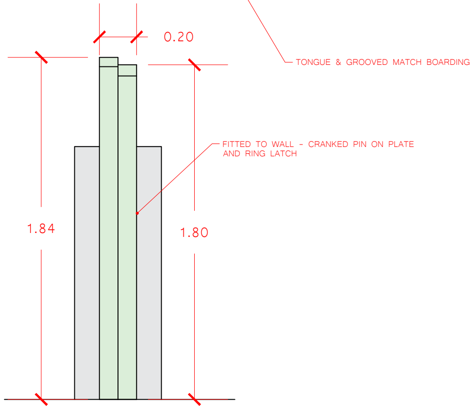
PROPOSED SOUTH-NORTH GATE SECTION
