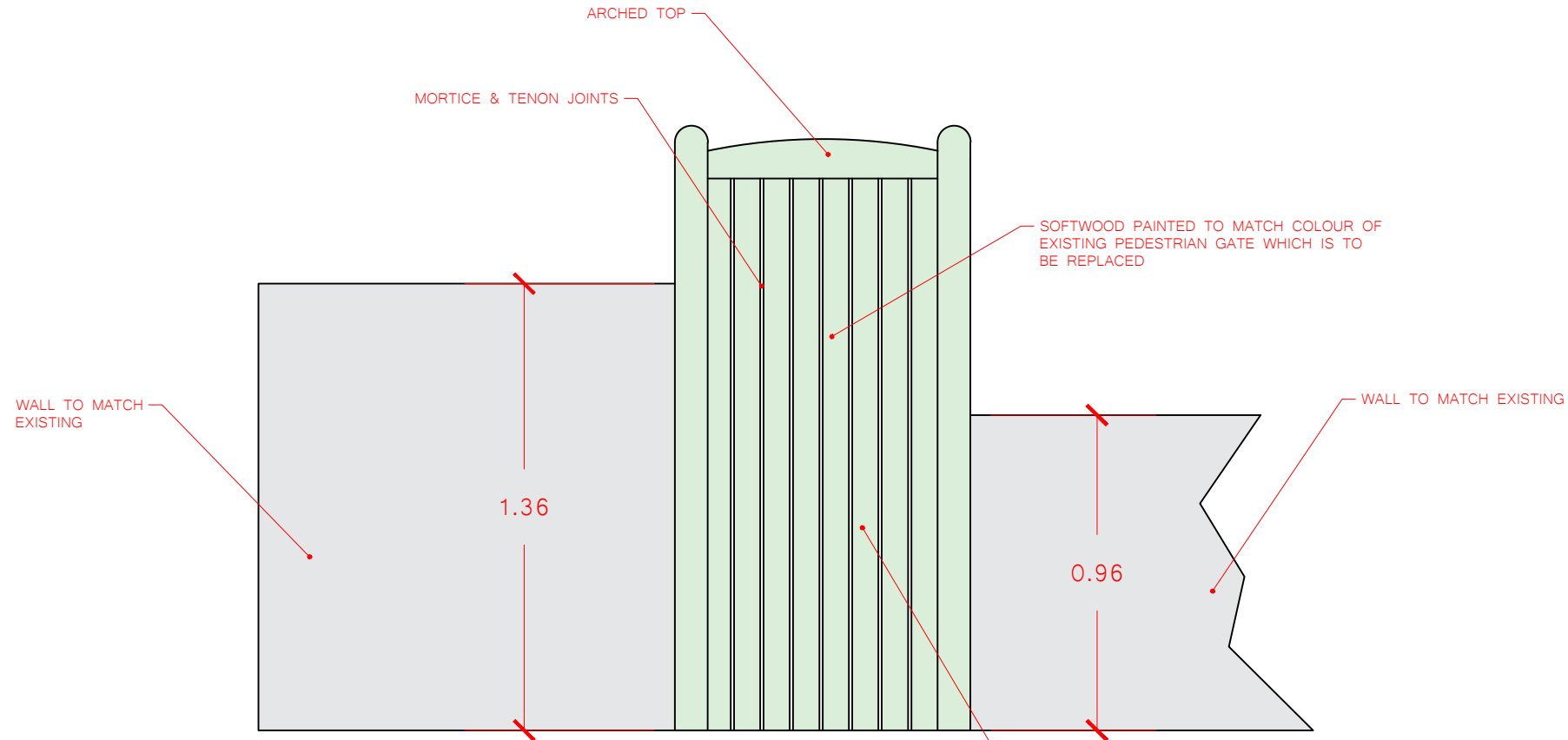
PROPOSED WEST-EAST GATE DETAIL
