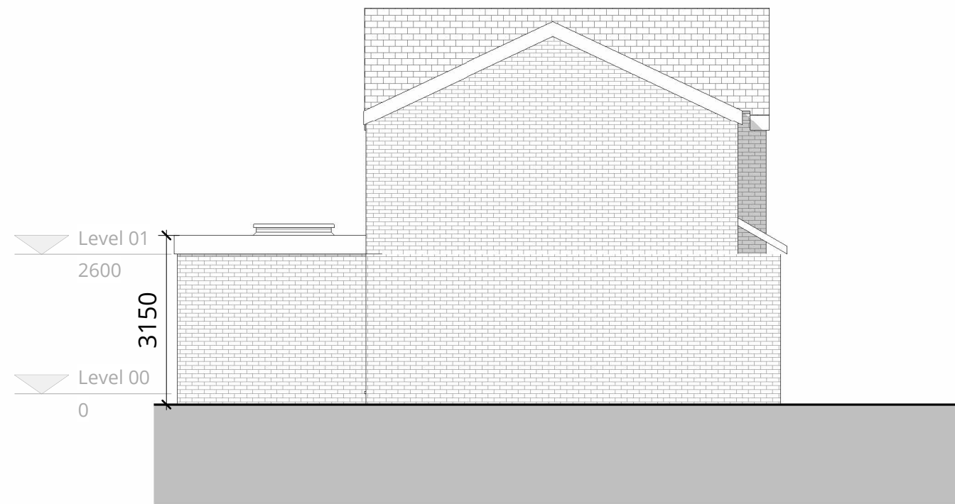
4 | Proposed Elevation Side 02 1:100
