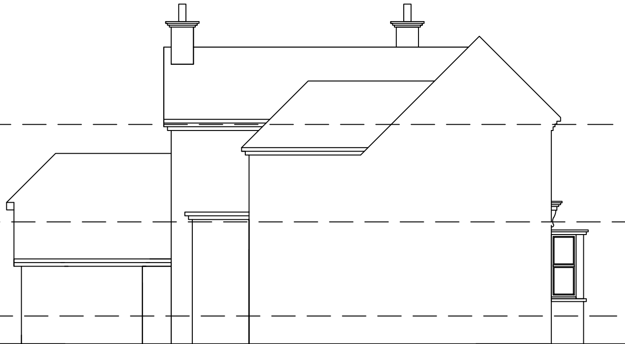
North-East Elevation
