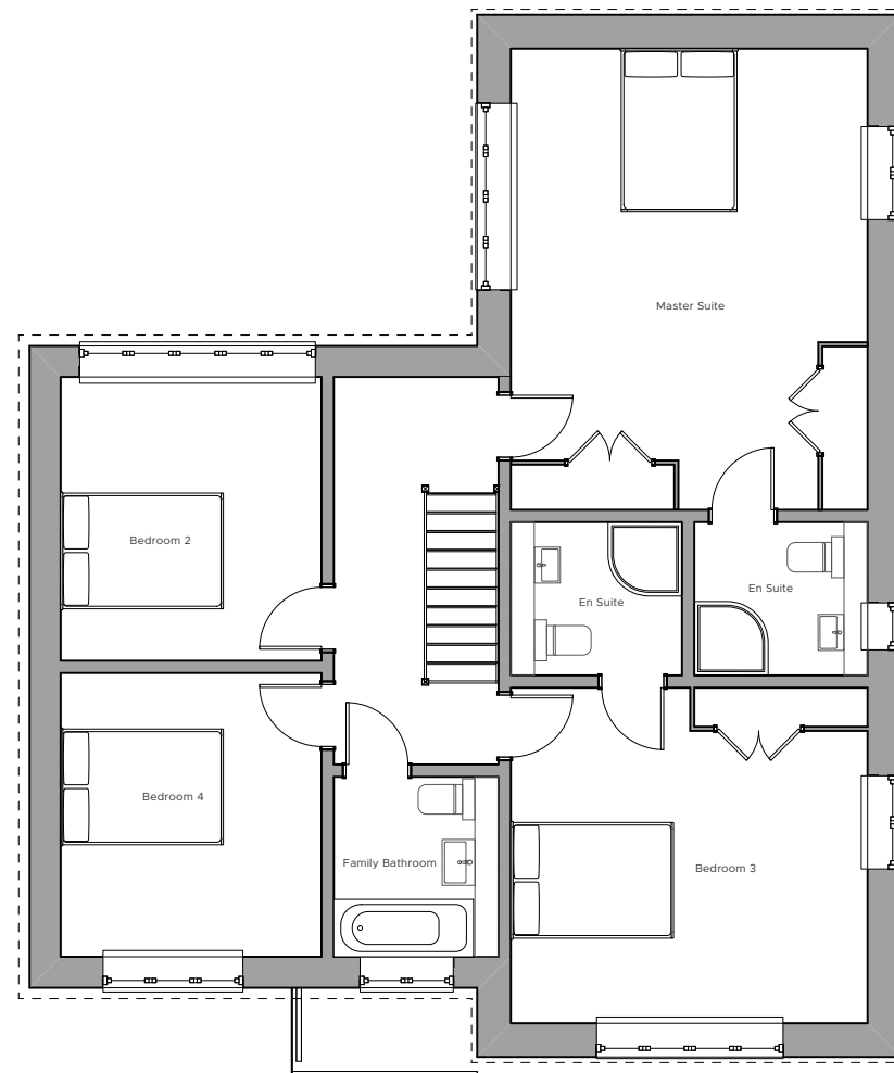
First Floor Plan Option 2 Scale: 1:100
