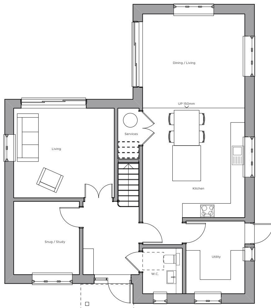
Ground Floor Plan Option 2 Scale: 1:100
