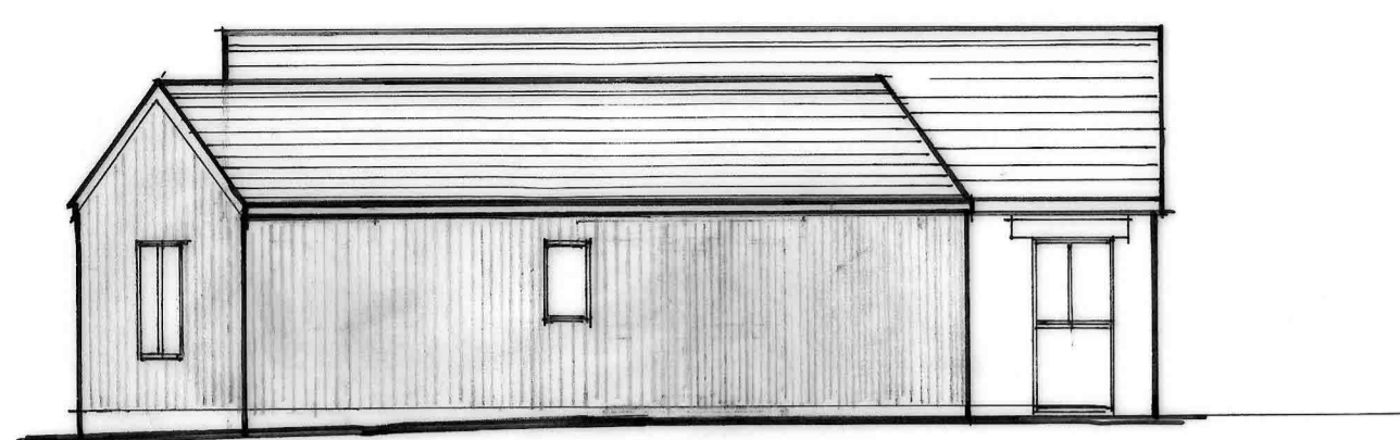
north east elevations
