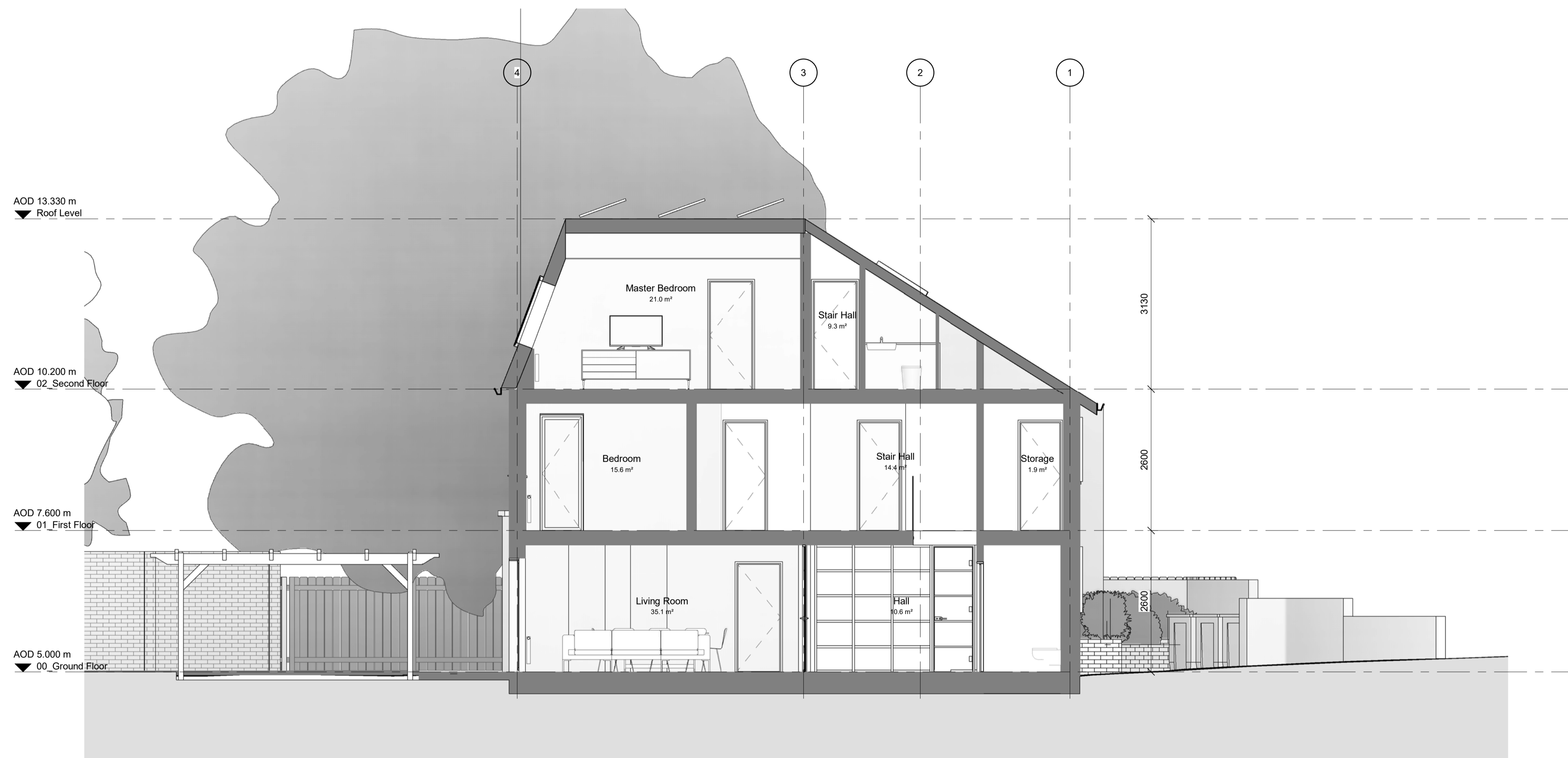
1 Proposed Section A-A 20350 1 : 50
