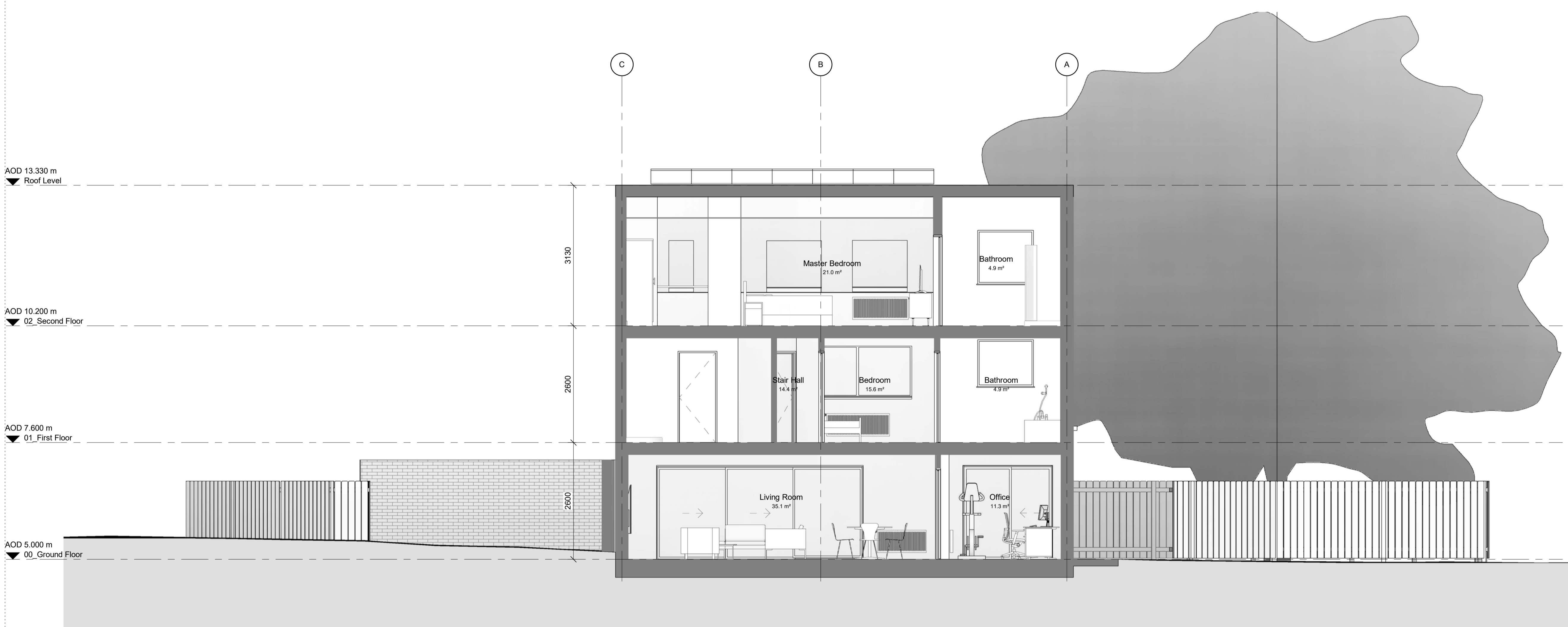
1 Proposed Section B-B 20351 1 : 50
